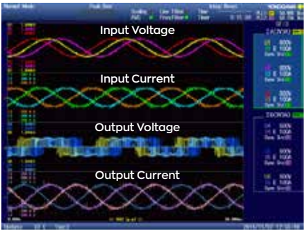
Matrix Drive Rated Power Operation
