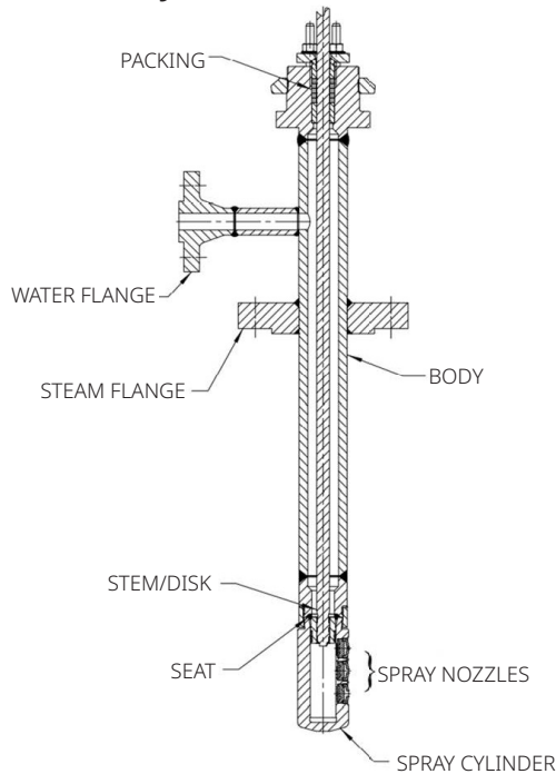
Figure 5. Yarway AT-38/48
