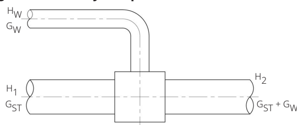
Figure 7. Yarway TempLow 4300
