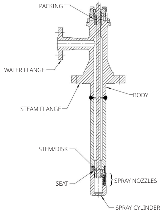
Figure 6. Yarway TempLow 4300
