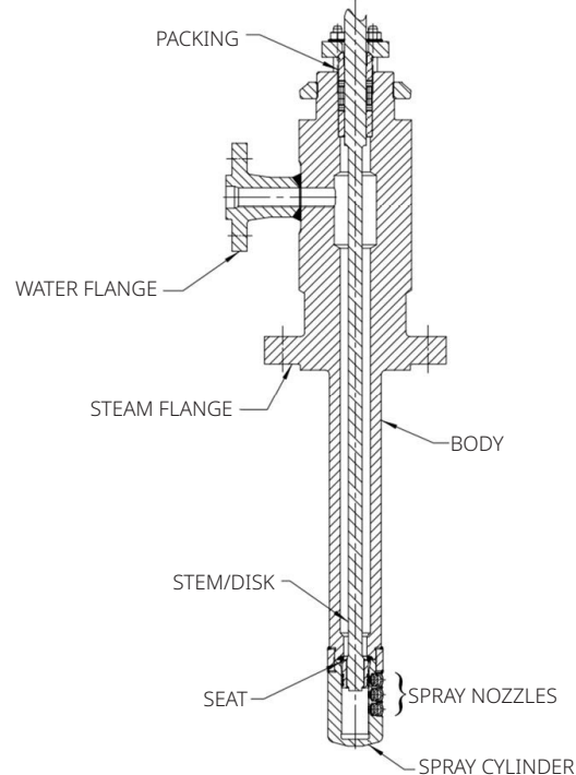
Figure 4. Yarway AT-18/28
