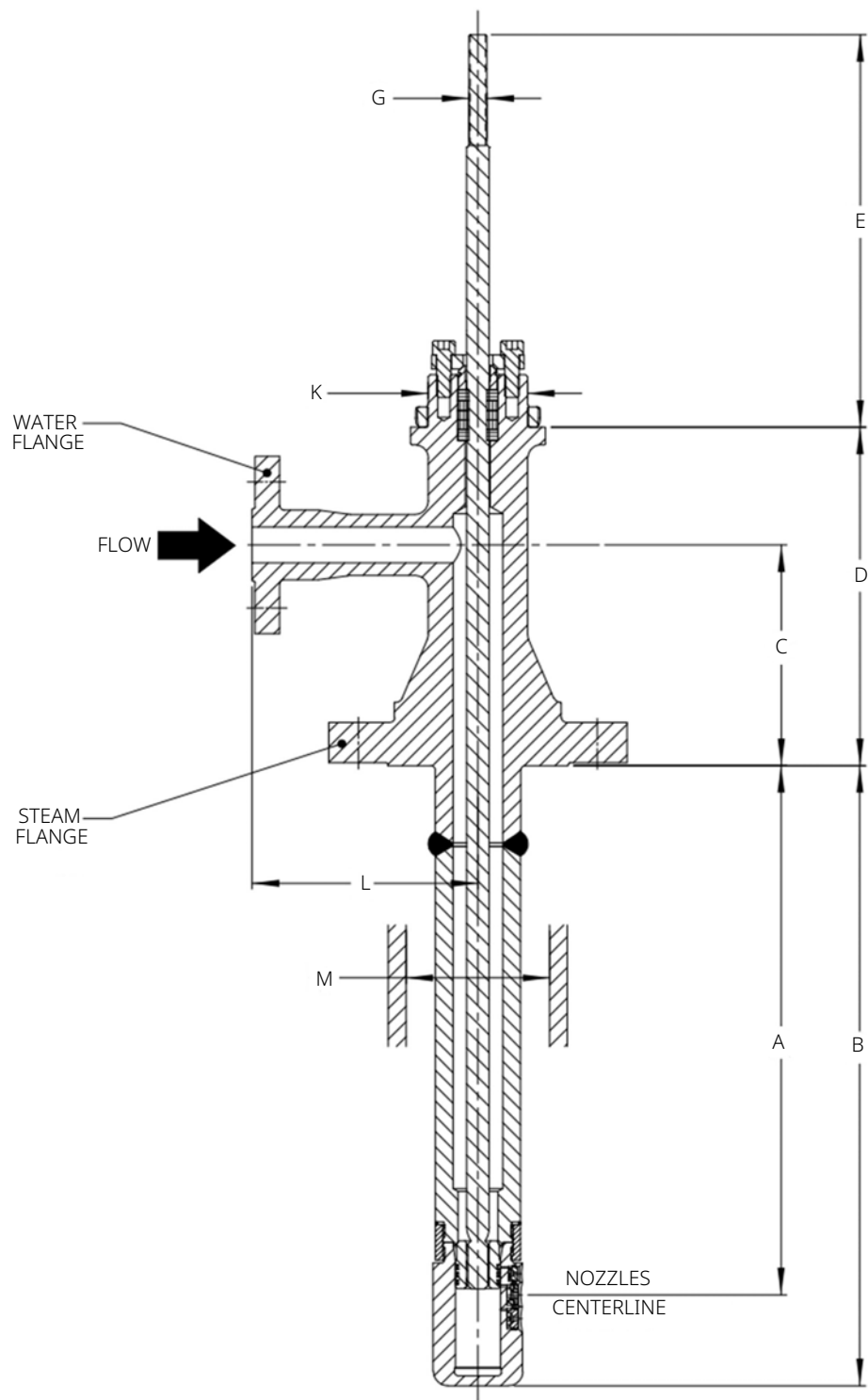
Figure 14. Yarway Templow 4300
