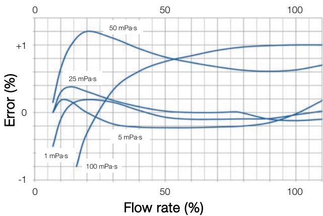
Effect of viscosity for liquids
