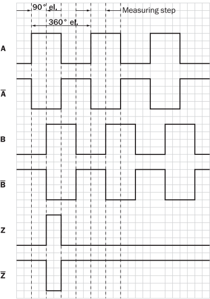
Cw with view on the encoder shaft in direction "A", compare dimensional drawing. ① Interfaces G, P, R only for channels A, B, Z.
