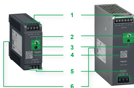
Compact housing 75 mm height (2.95 in)
