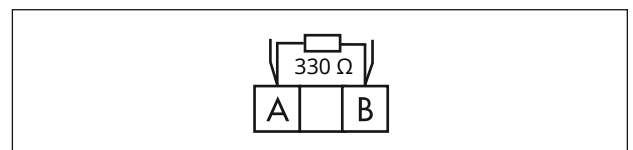
Fig. 22: RS-485 interface with external bus termination
