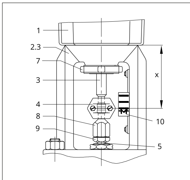
Fig. 9: Mounting on Series 240 Valves
