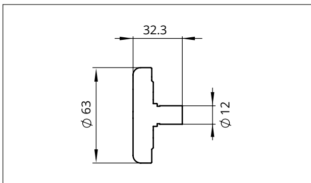
Fig. 28: Dimensions in mm · Handwheel as special version
