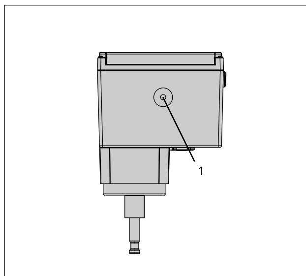
Fig. 8: Actuating shaft for manual override (version with ring nut)
