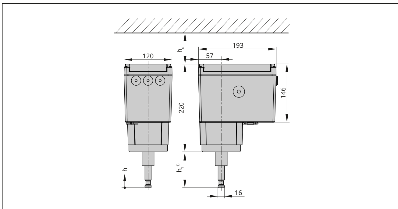
Fig. 25: Dimensions in mm · Type 3374-15, -17, -26 and -36 (form A)
