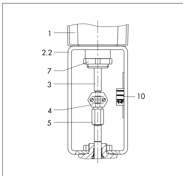
Fig. 10: Mounting on Type 3214
