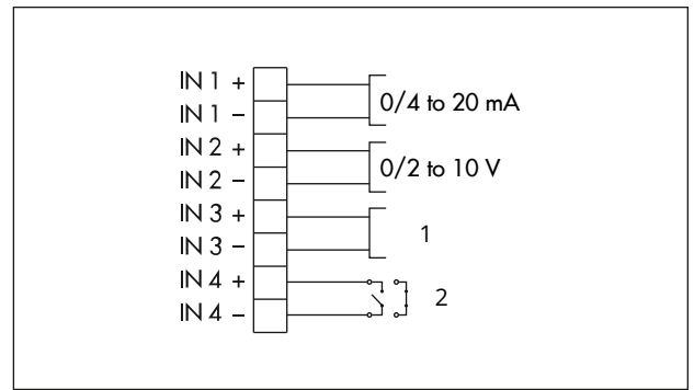
Fig. 20: Terminal assignment for 'Temperature closed-loop control upon input signal failure' application
