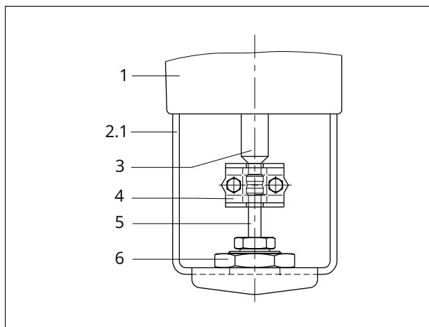
Fig. 5: Mounting · Version with integrated yoke
