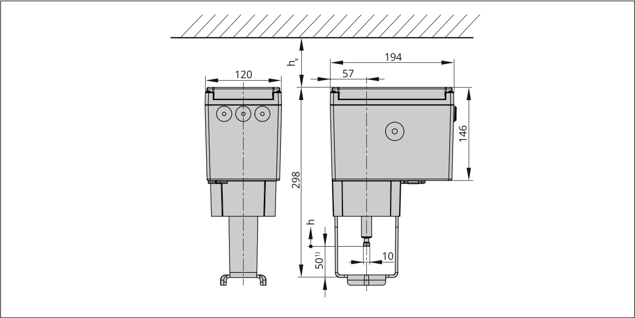
Fig. 24: Dimensions in mm · Type 3374-10, -11, -21 and -31 (form B)
