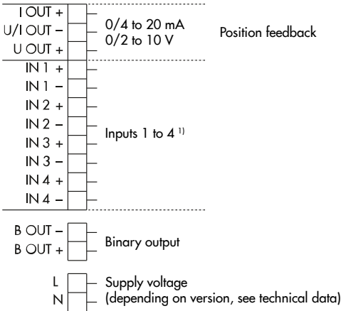
Fig. 14: Electrical connection
