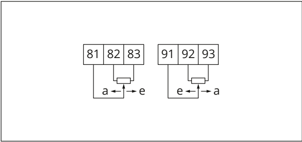
Fig. 13: Resistance transmitter
