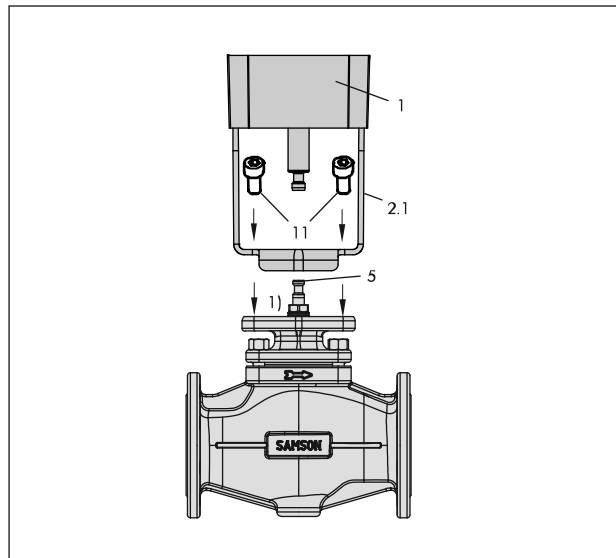
Fig. 6: Mounting · Version with actuator yoke and V2001 accessories
