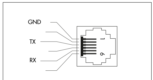
Fig. 23: Assignment of the RJ-12 jack
