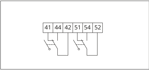
Fig. 12: Mechanical limit contacts
