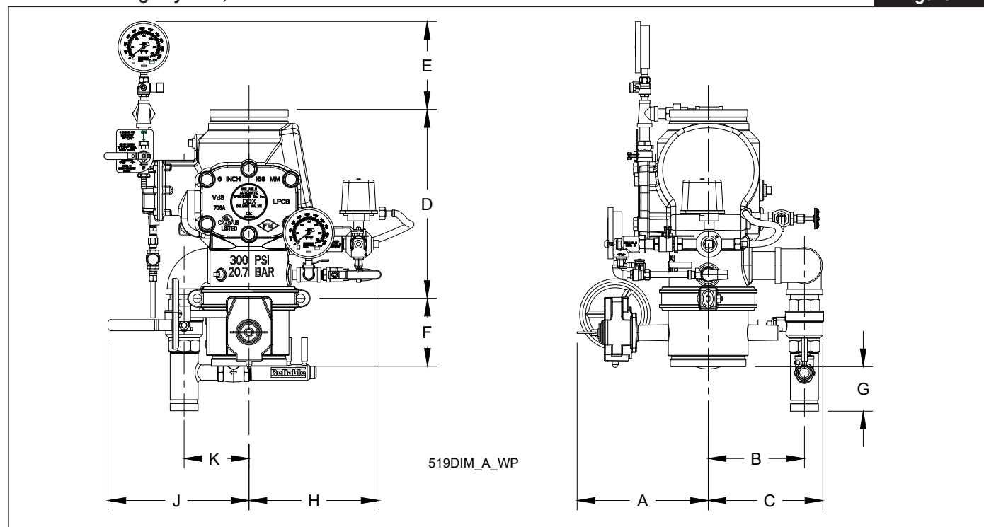
Model DDX Deluge System, Wet Pilot Line Release Trim
