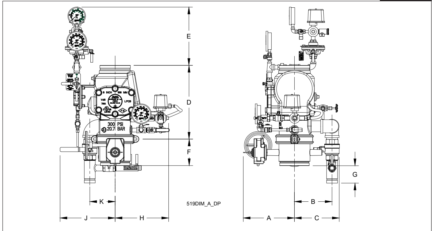
Model DDX Deluge System, Dry Pilot Line Release Trim
