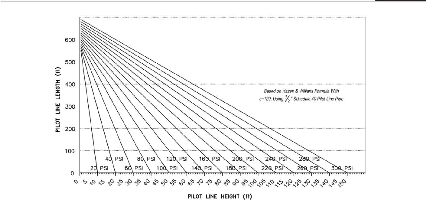
Wet Pilot Line Height vs. Length
