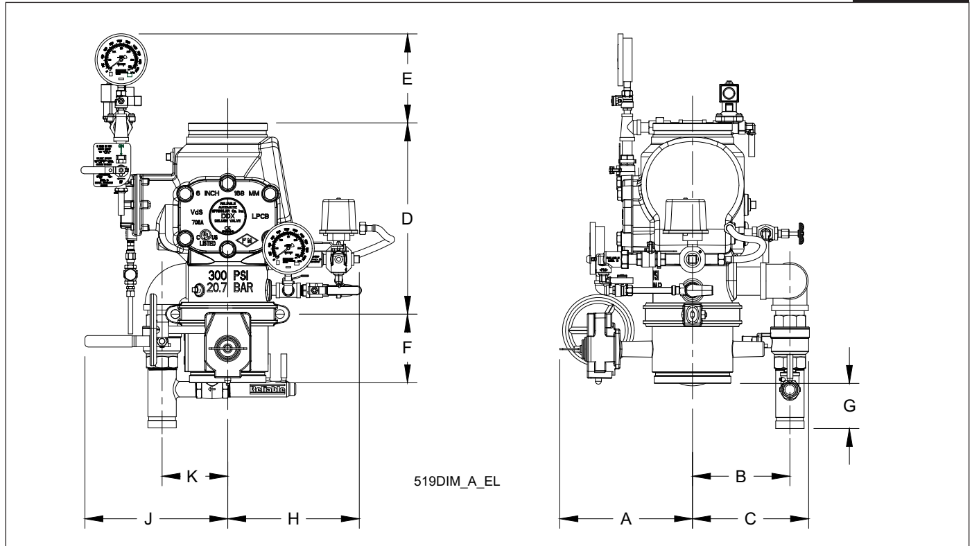
Model DDX Deluge System, Electric Release Trim
