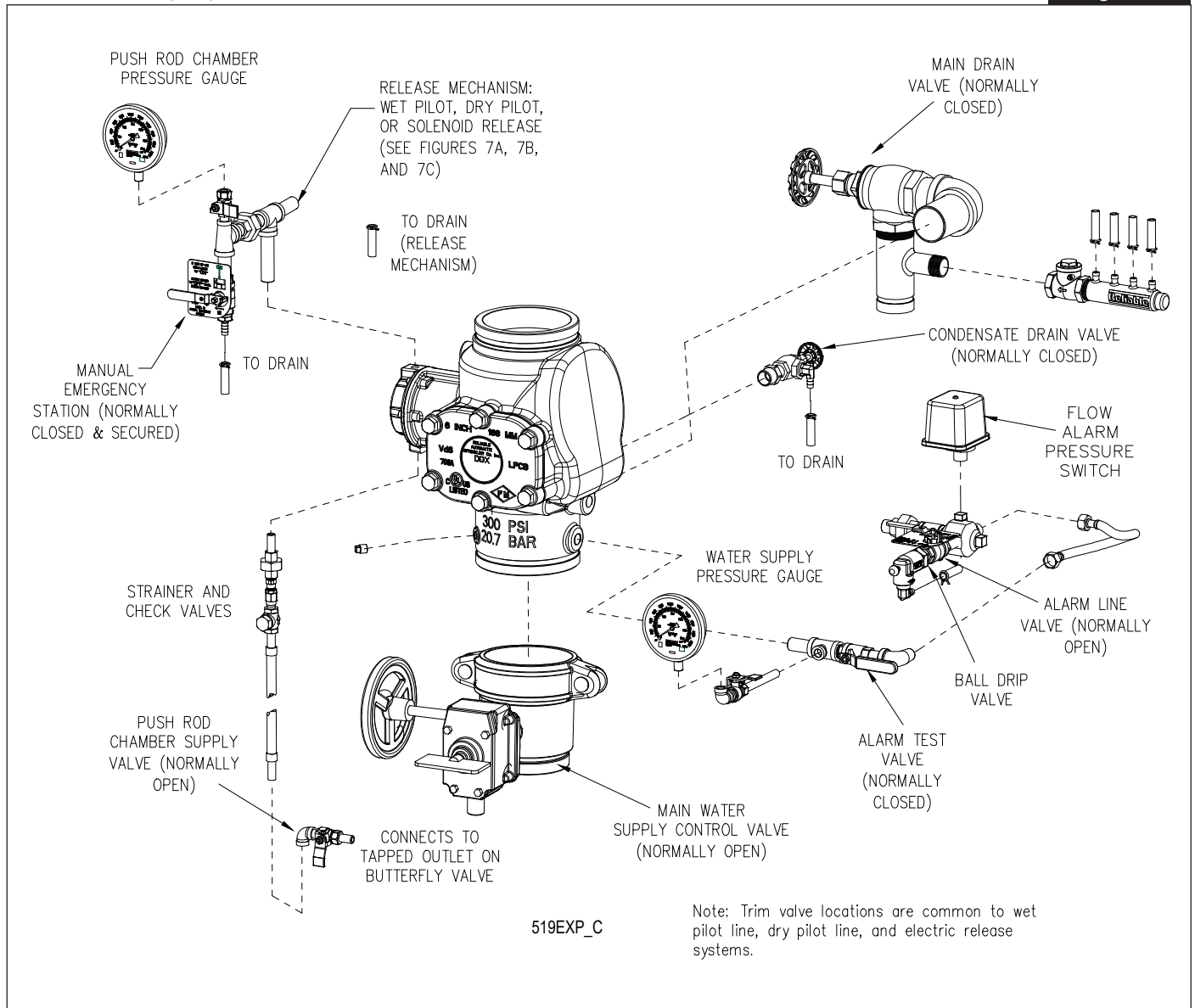
Model DDX Deluge System Components
