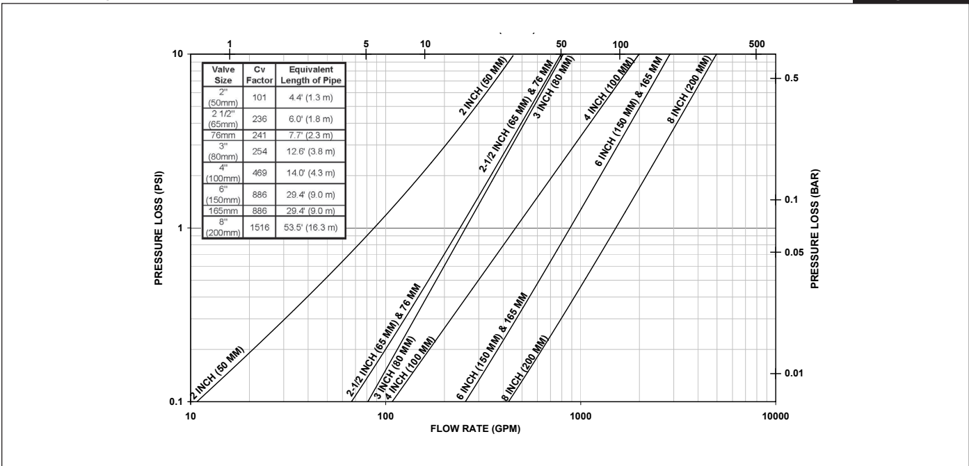
Model DDX Hydraulic Friction Loss Graph
