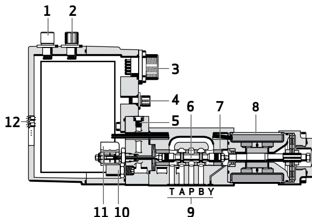
D638 Series Direct Drive Servo Valve
