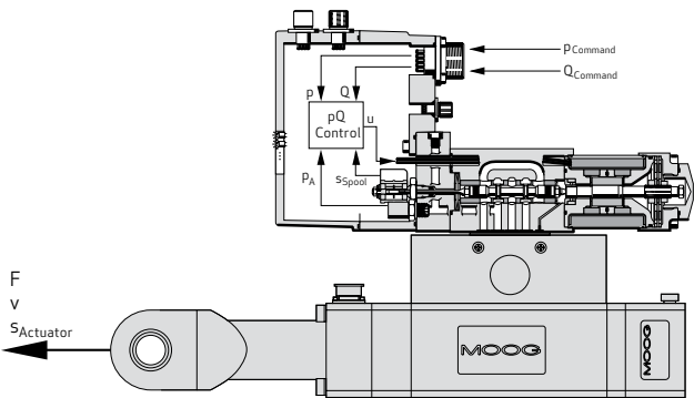
Control loop consisting of valve with integrated pQ control and cylinder
