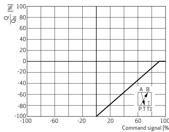
Flow signal characteristic - in bypass line
