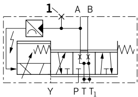
4-way valve in main line
