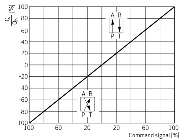
Flow signal characteristic - in main line
