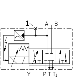
3-way valve in main line
