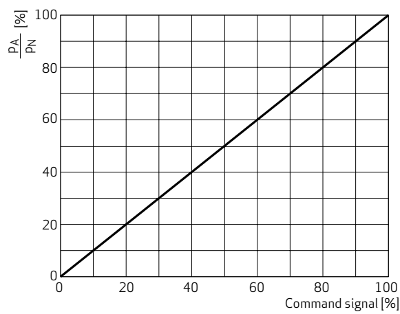
Pressure signal characteristics
