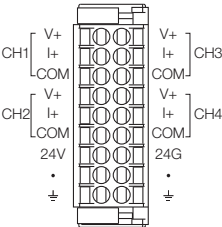
FX5-4DA
