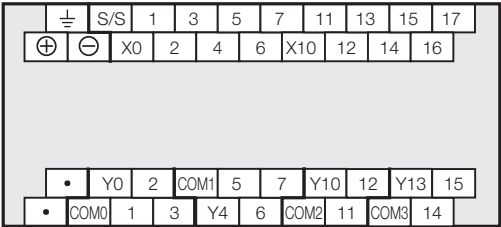
FX5S-30MT/DSS
