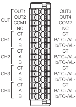
FX5-4LC
