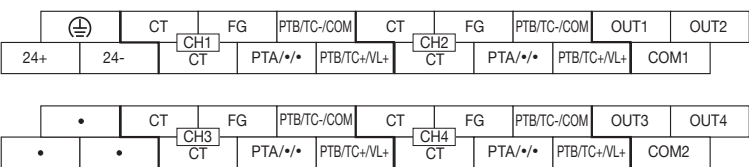
FX3U-4LC
