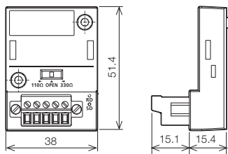
FX5-SDCD
