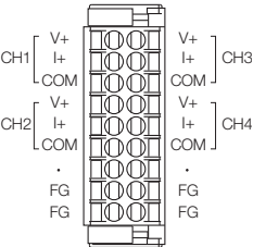
FX5-4AD
