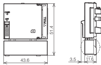
FX5-SDCD
