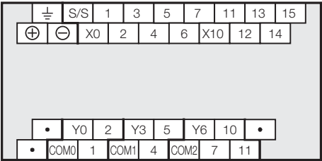
FX5UJ-24MT/DSS
