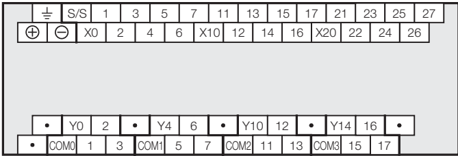
FX5S-40MT/DSS
