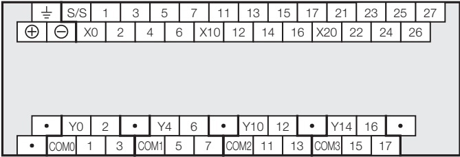
FX5UJ-40MT/DSS
