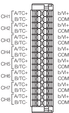
FX5-8AD
