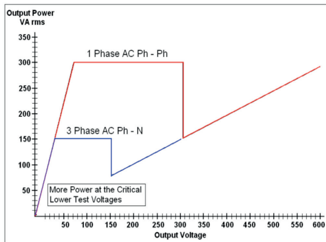
Figure 4: Voltage output power curve
