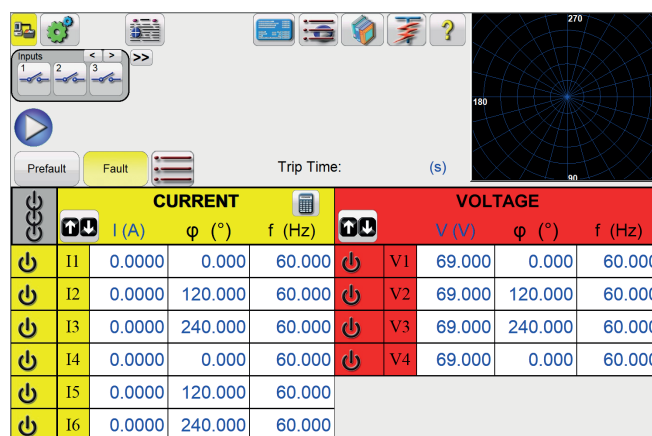
Figure 2: STVI advanced user interface
