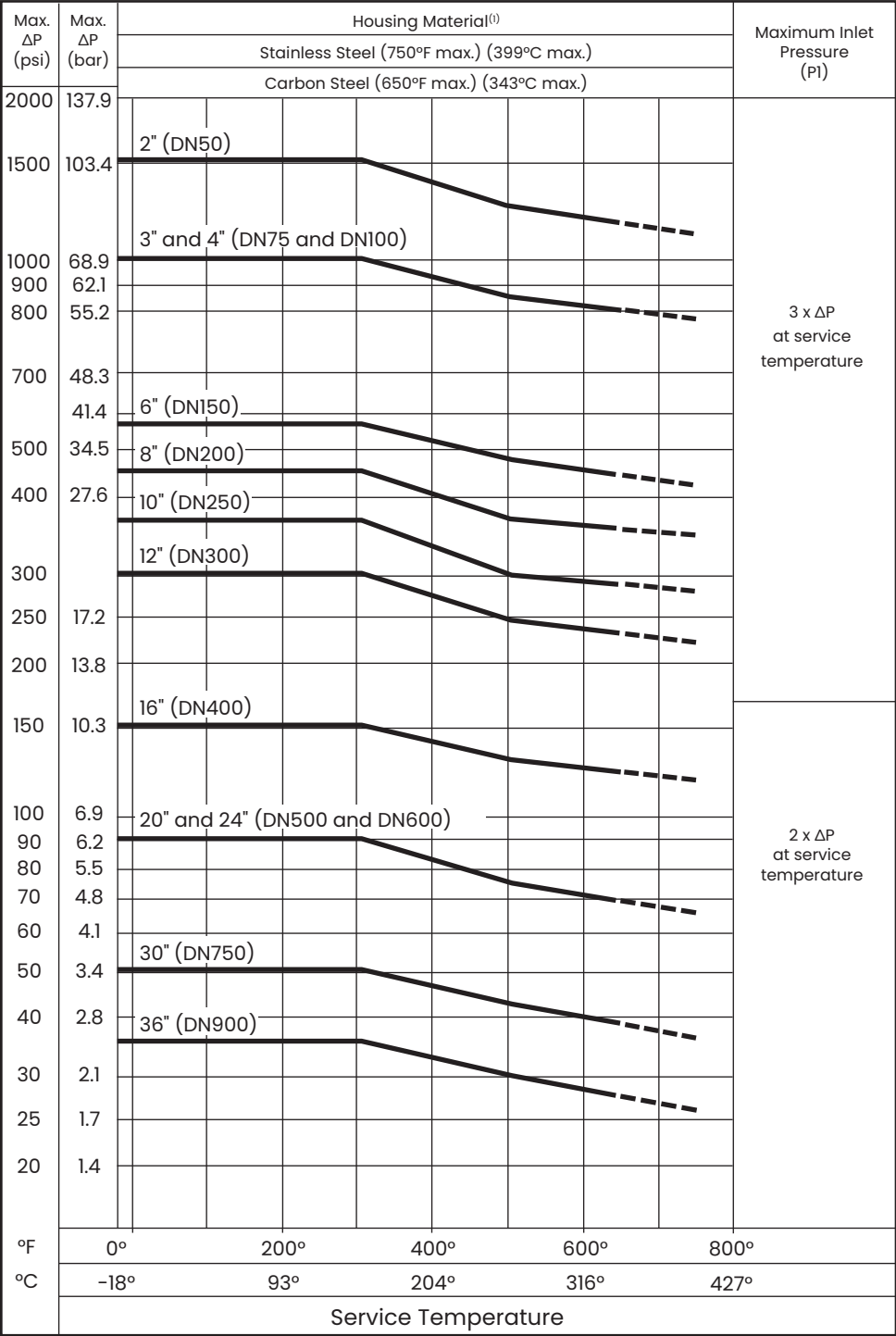
Pressure Drop vs. Temperature (2) (3)
