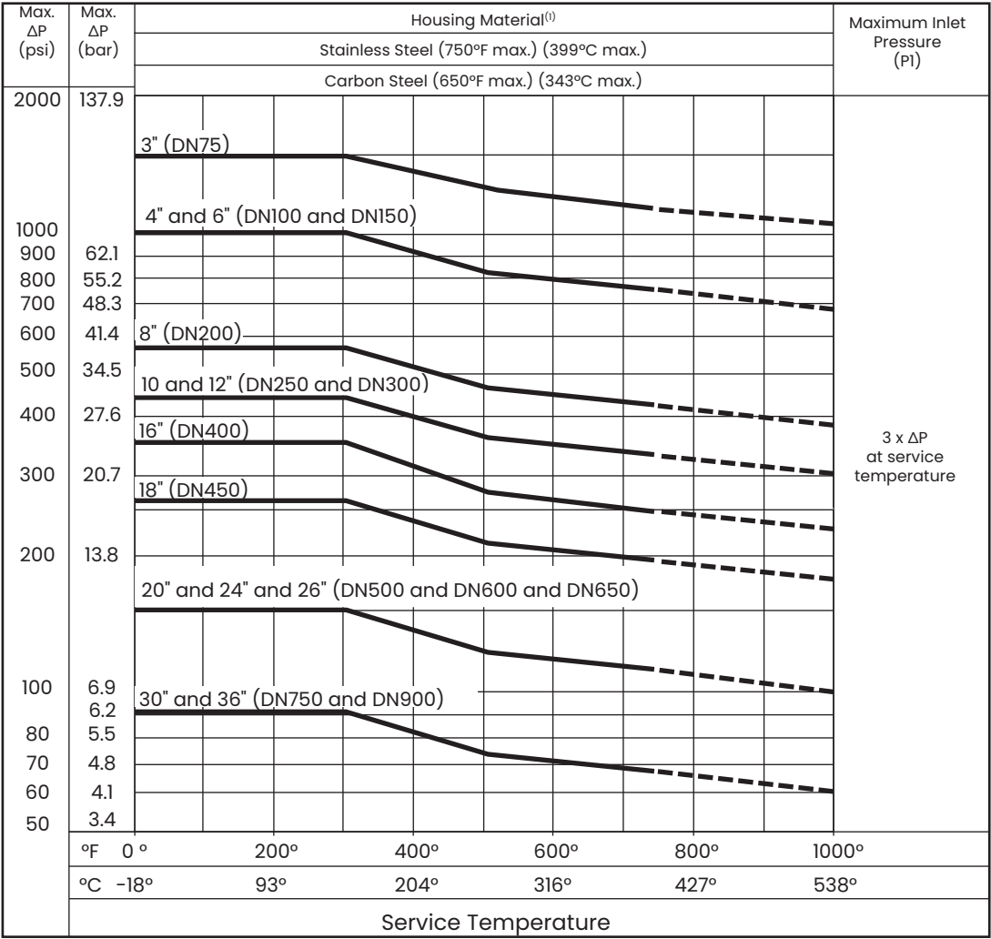
Pressure Drop vs. Temperature (2)
