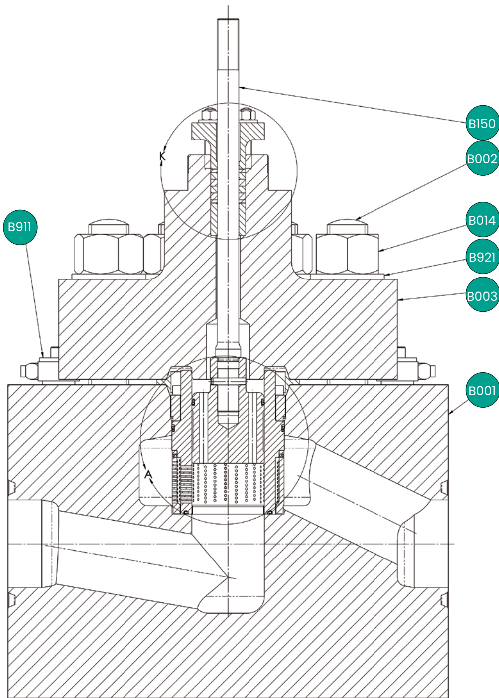
Cross Sectional View of 41005 API 6A Design
