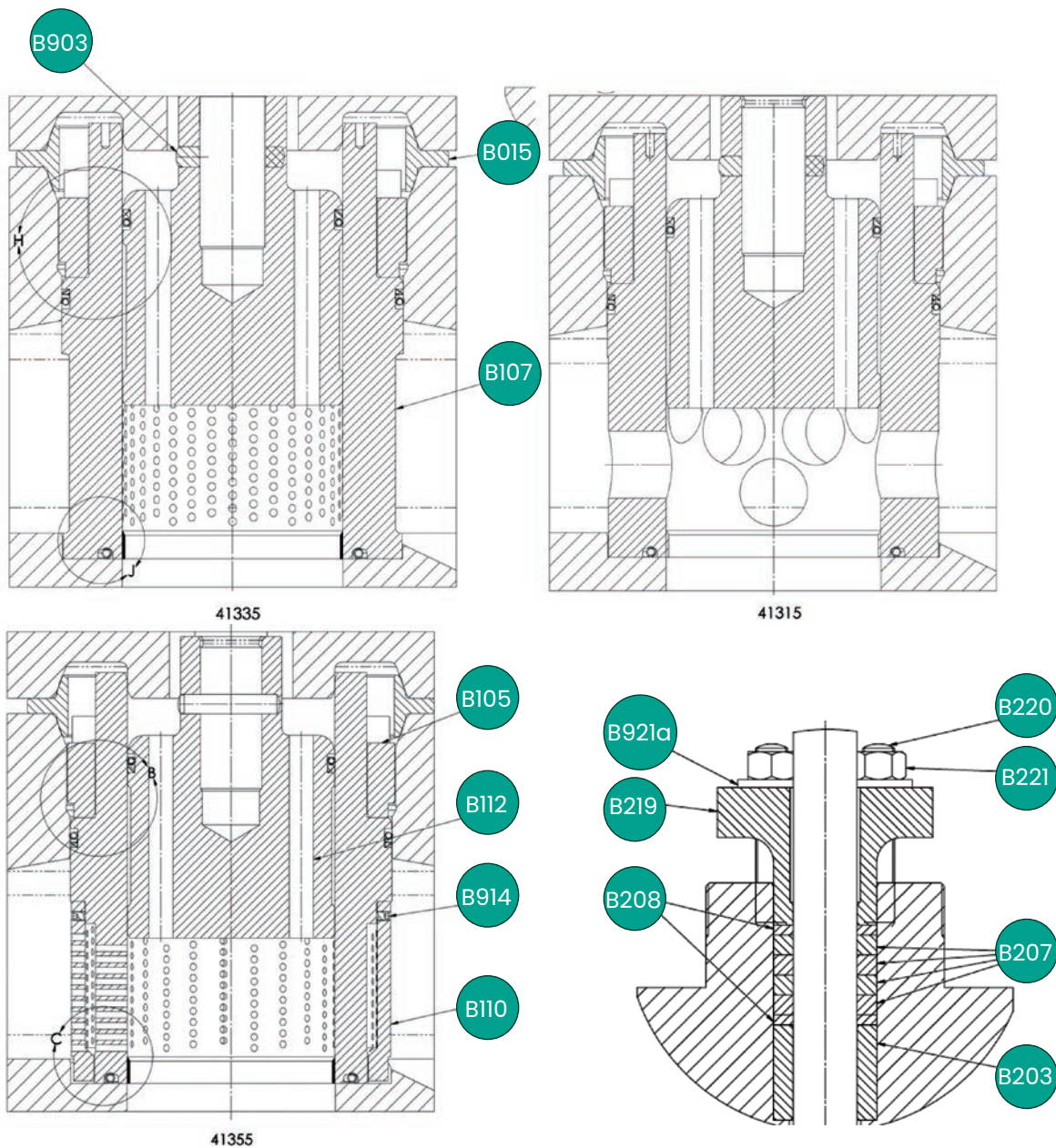
Trim Type and Packing Detail
