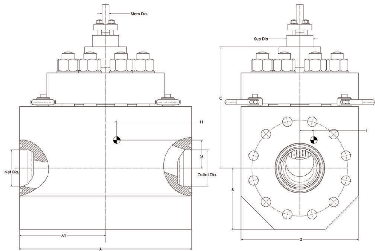
API 10K and 15K Body Sub-Assembly dimensions (inches)
