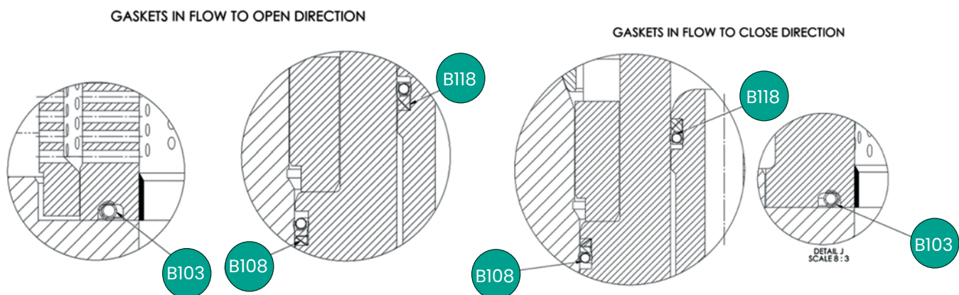
Trim Gaskets Detail
