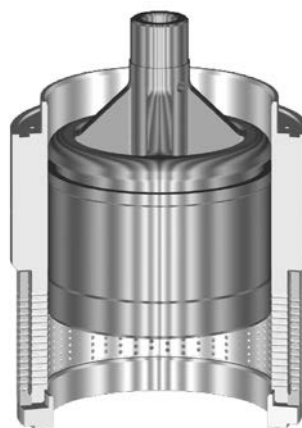
Models 41355 - 41555 - 41655 - 41755 - 41955 Multi-Stage Low Noise Trim FTO
