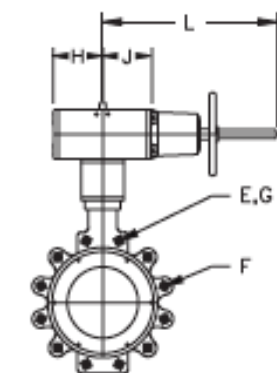
Double Acting Sizes 210 thru 280
