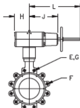
Spring Return Sizes 210/230/250/270
