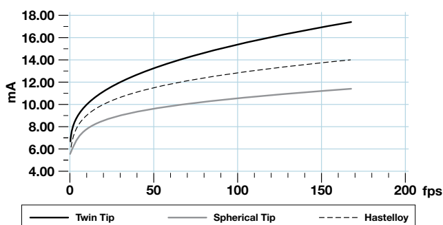
Typical Air Flow
