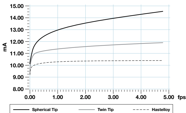
Typical Water Flow
