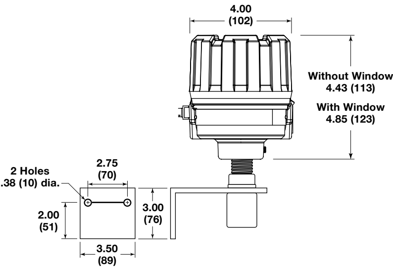
Model TD2 with Remote Electronics
