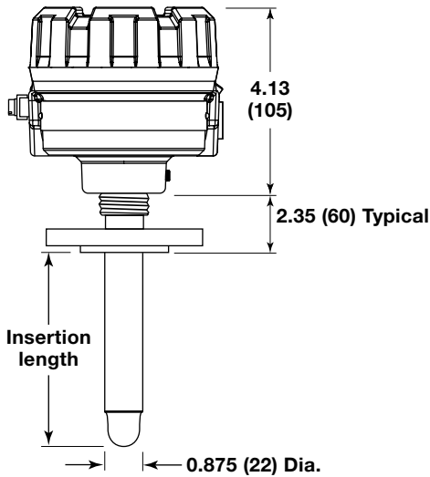
Remote Spherical Tip Probe with Flange Connection
