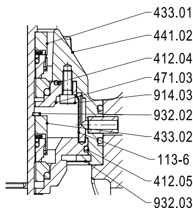
Fig. 23: Double mechanical seals 5A/M7N, tandem arrangement, unbalanced, non-drive end (shaft unit DW40.1)
