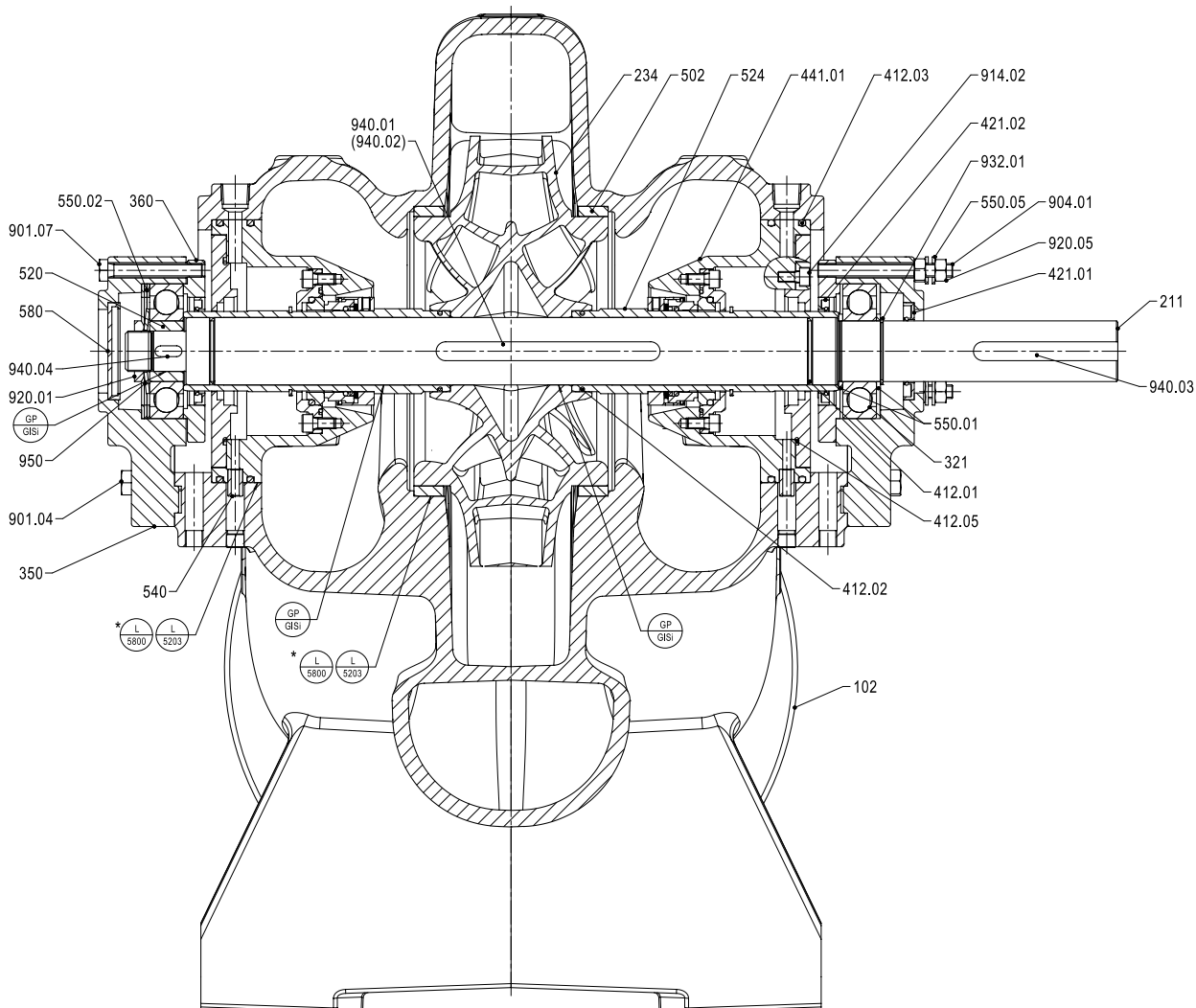
Fig. 7: General assembly drawing of Omega / Omega V (Generation 2), horizontal installation 3E
