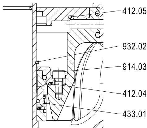
Fig. 18: Single mechanical seals 5A/M7N/M74, unbalanced, drive end
