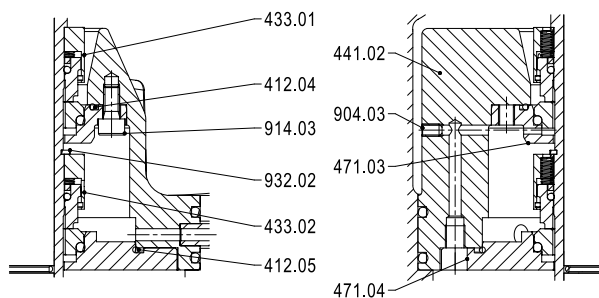
Fig. 19: Double mechanical seals 5A/M7N/M74, tandem arrangement, unbalanced, non-drive end
