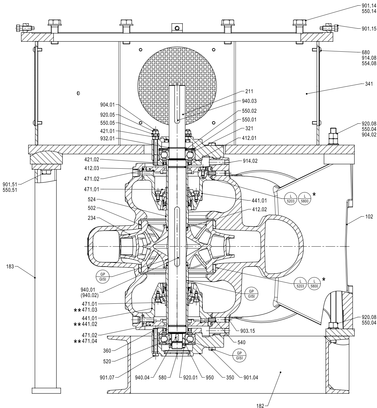
Fig. 15: General assembly drawing of Omega / Omega V (Generation 2), vertical installation DB/DK
