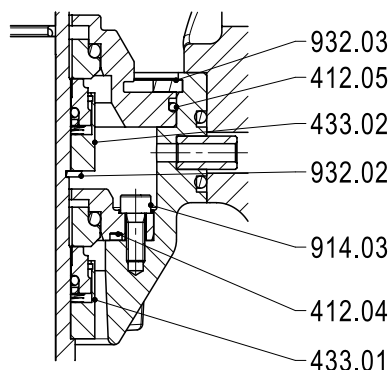
Fig. 22: Double mechanical seals 5A/M7N, tandem arrangement, unbalanced, drive end (shaft unit DW40.1)
