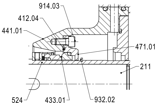
Fig. 9: Single mechanical seals 5A/M7N/M74, standard design, unbalanced
