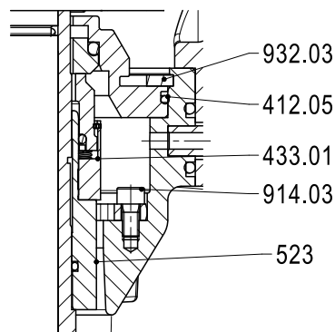
Fig. 24: Single mechanical seal 5BOM, balanced, drive end (shaft unit DW40.1)
