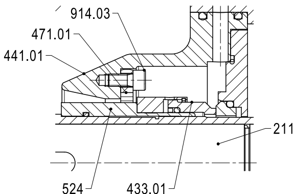
Fig. 11: Standard variant: Mechanical seal 5BOM, balanced
