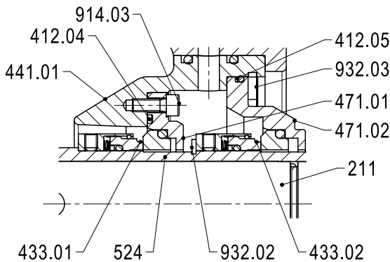
Fig. 13: Double mechanical seals 5A/M7N, tandem arrangement, unbalanced (shaft unit DW40.1)
