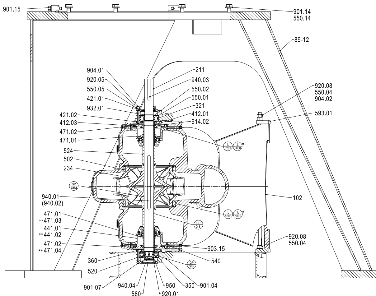
Fig. 16: General assembly drawing of Omega / Omega V (Generation 2), vertical installation DM
