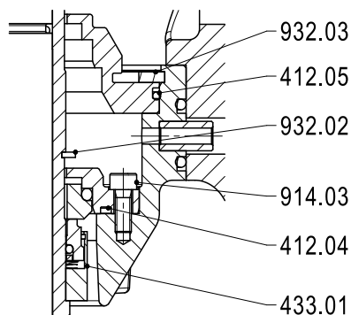
Fig. 21: Single mechanical seals 5A/M7N, unbalanced, drive end (shaft unit DW40.1)
