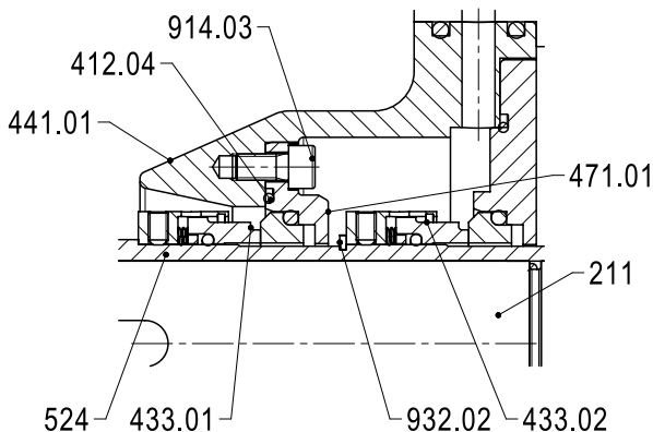
Fig. 10: Double mechanical seals 5A/M7N/M74, tandem arrangement, unbalanced
