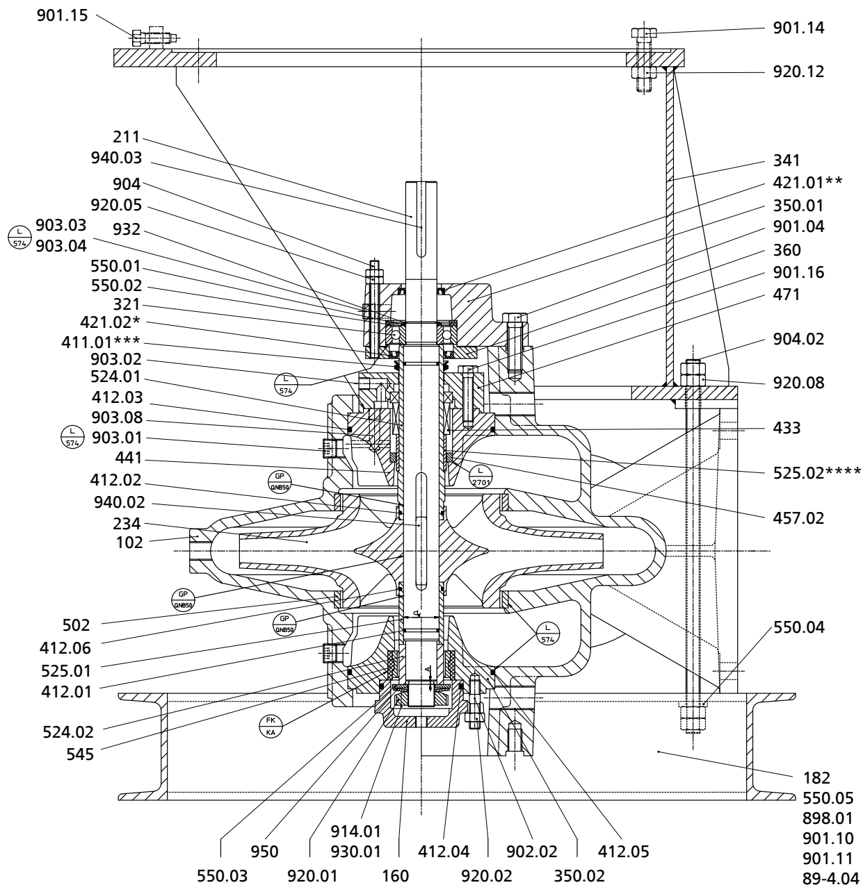
Fig. 6: General assembly drawing of Omega / Omega V (Generation 1), installation type DB
