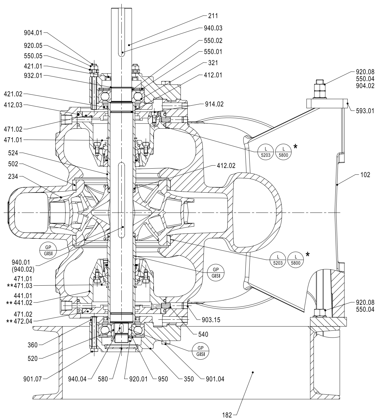
Fig. 14: General assembly drawing of Omega / Omega V (Generation 2), vertical installation DJ
