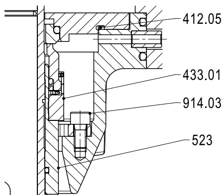
Fig. 20: Single mechanical seal 5BOM, balanced, drive end
