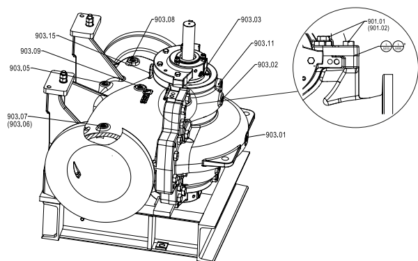
Fig. 17: Vertical installation: Position of hexagon head bolts and screw plugs
