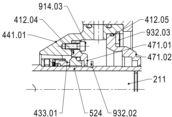
Fig. 12: Single mechanical seals 5A/M7N, standard design, unbalanced (shaft unit DW40.1)
