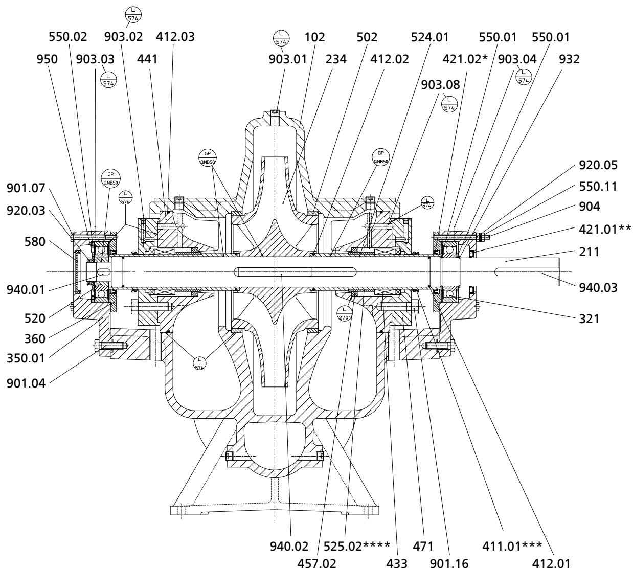
Fig. 5: General assembly drawing of Omega / Omega V (Generation 1), horizontal installation
