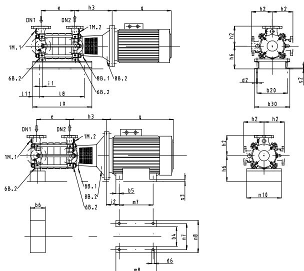
Fig. 6: Multitec E dimensions
