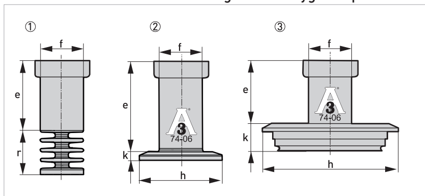
Figure 2-3: Dimensions for pressure transmitter with cooling fins and hygienic process connections
