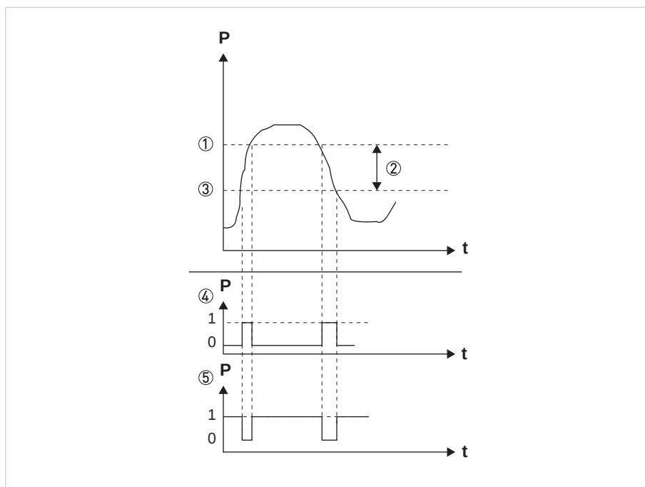
Figure 4-2: Switching output signals (window function)
