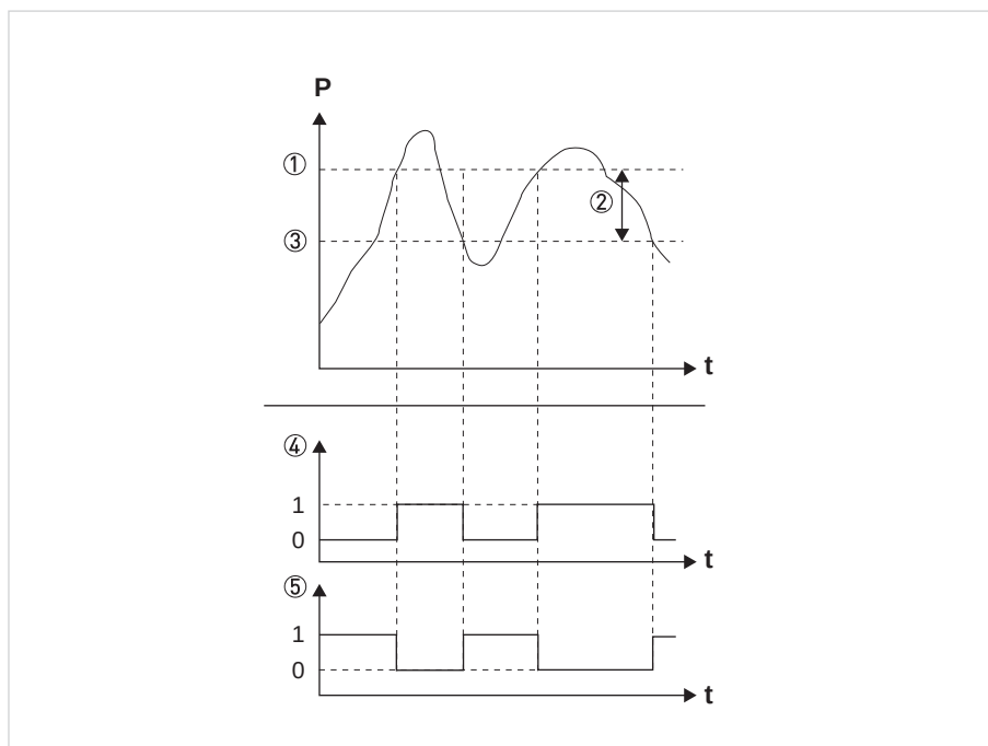
Figure 4-3: Switching output signals (hysteresis-function)
