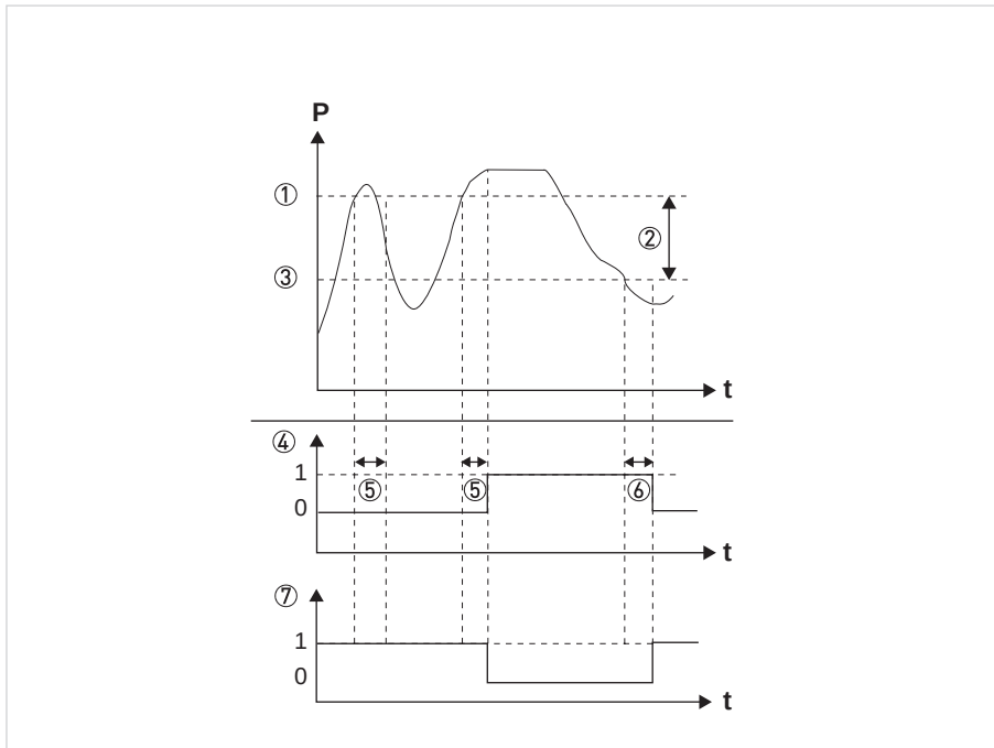
Figure 4-4: Switching output signals (hysteresis-function with damping)
