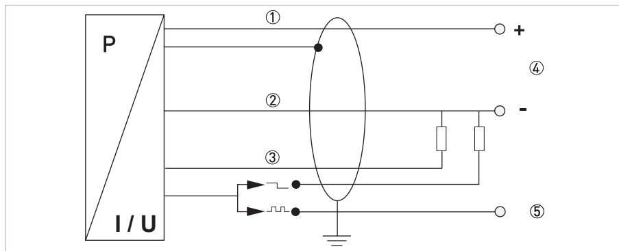
Figure 4-1: Electrical connection diagram 2-wire 4...20 mA
