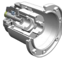
Magnetic coupling
