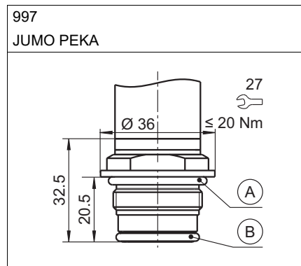
A O-ring 26 × 2.5 B O-ring 21 × 2.5
