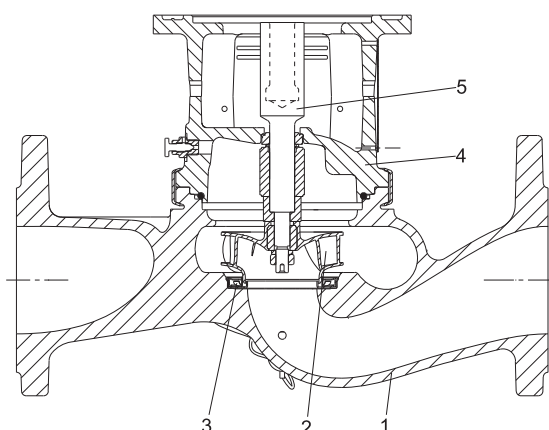
Sectional drawing of a TPE2 Small pump
