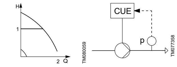
Constant pressure with stop function, difference between start and stop pressures (ΔH)
