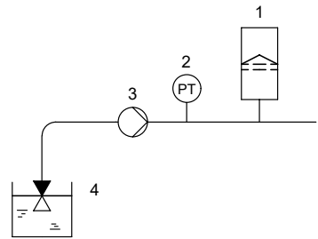
Position of the non-return valve and pressure sensor in a system with suction lift
