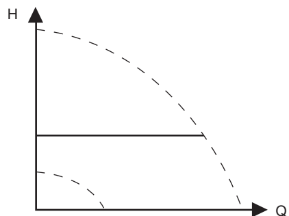
Constant differential pressure
