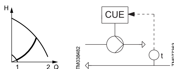
Constant temperature
