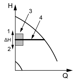
Constant pressure with stop function, difference between start and stop pressures (ΔH)
