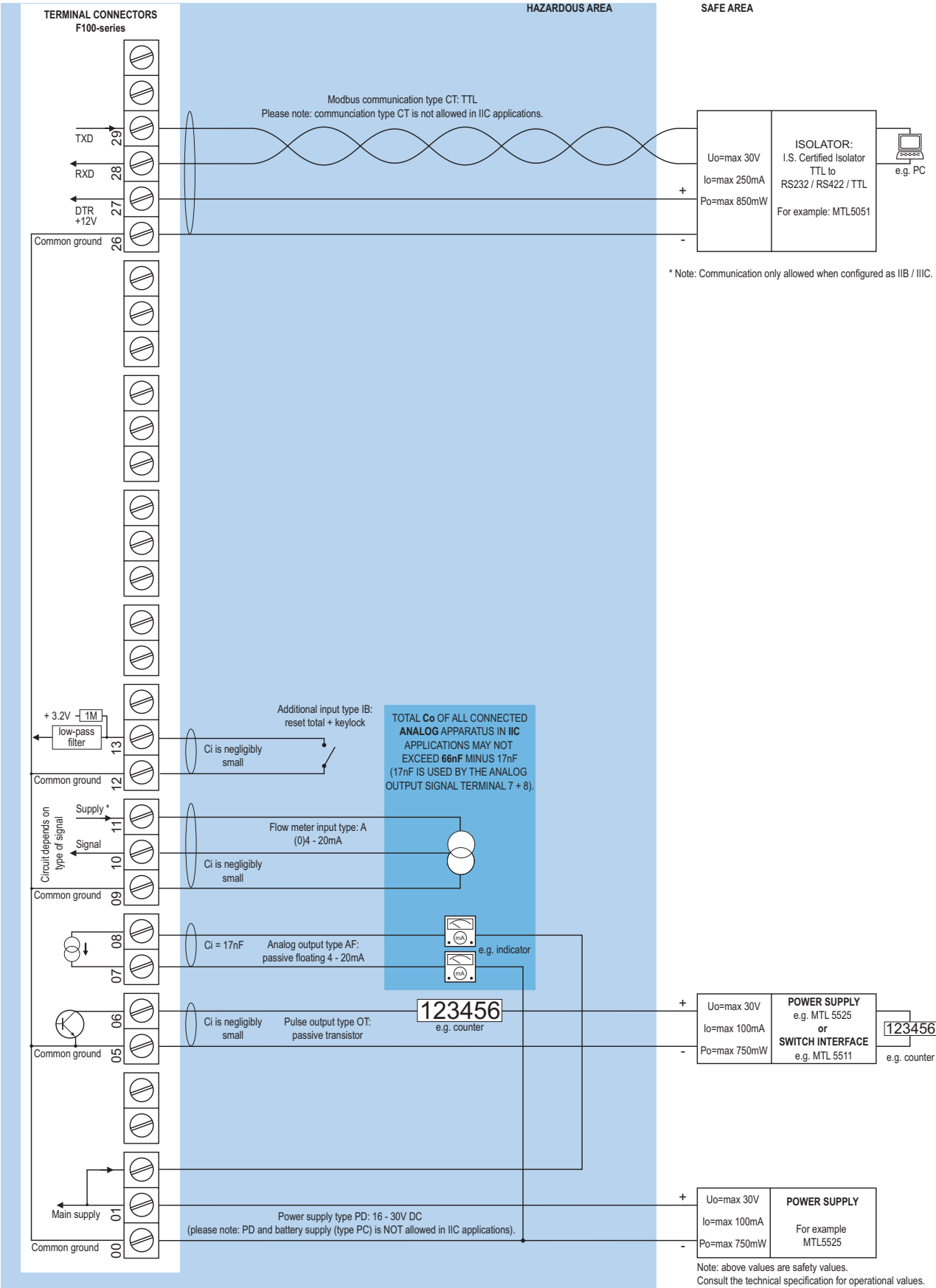
Configuration example IIB / IIIC and IIC - F110-A-AF-(CT)-IB-OT-PD-XI - Power requirement 16 - 30V DC
