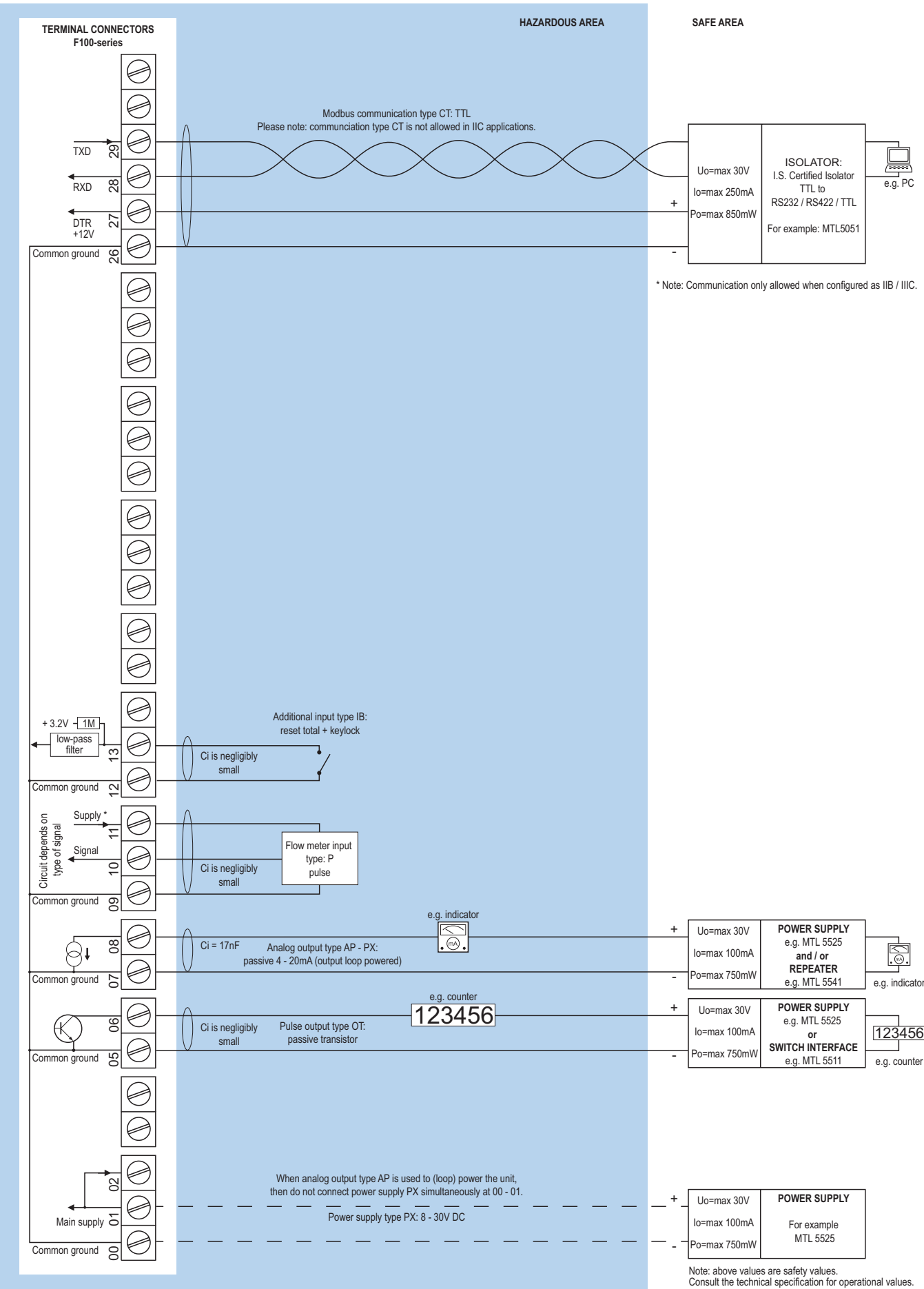
Configuration example IIB /IIC and IIC - F110-P-AP-(CT)-IB-OT-(PX)-XI - Output loop powered
