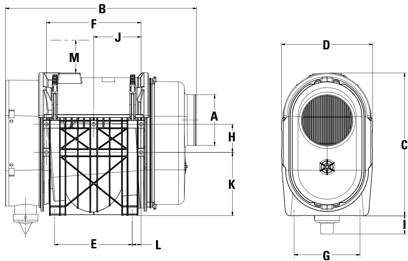
PSD14 — Service Access on Side (Vertical Model Shown)
