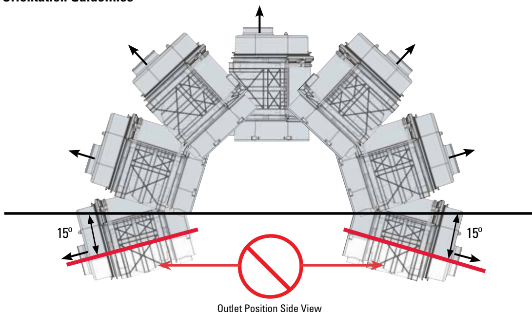
Outlet Position Side View
