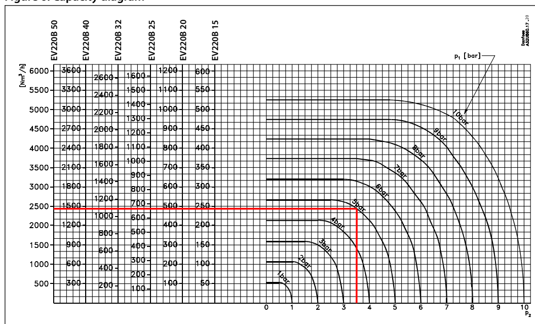
Figure 6: Capacity diagram
