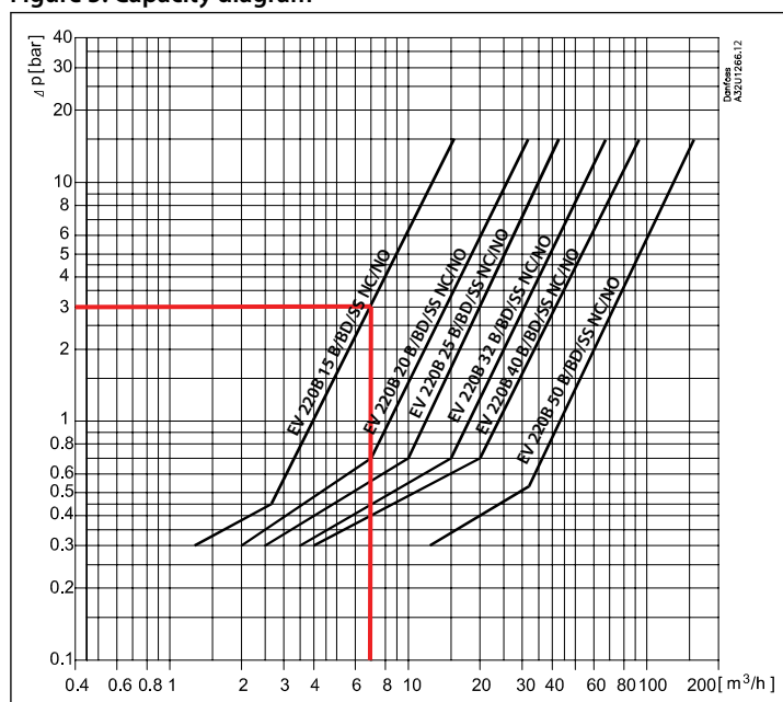
Figure 5: Capacity diagram
