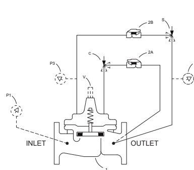
SINGLE CLOSING LINE
