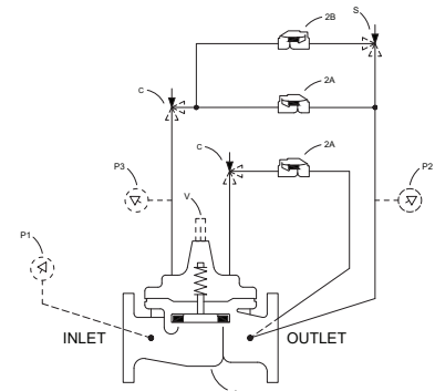
DUAL CLOSING LINE
