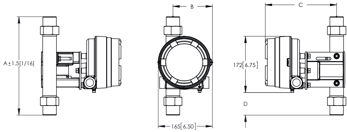
Model 3809 Explosion Proof Indicator Housing with Threaded Female Connections mm [inches]
