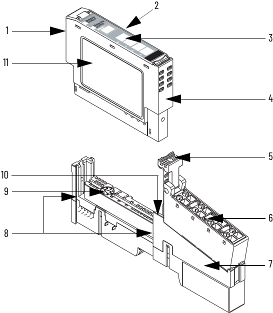
Figure 1 - POINT I/O Module with 1734-TB or 1734-TBS Wiring Base Assembly
