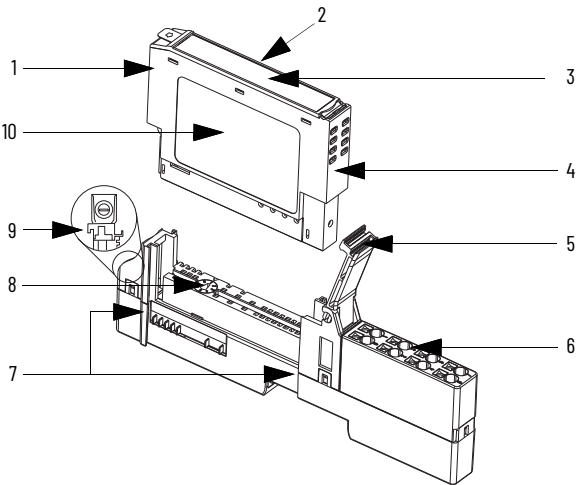
Figure 2 - POINT I/O Module with 1734-TOP or 1734-TOPS One-piece Terminal Base
