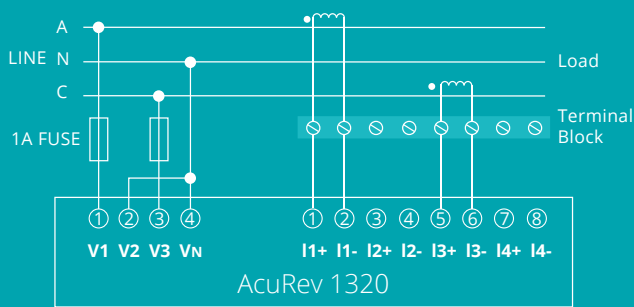
2 ELEMENT 3 WIRE 1 PHASE
