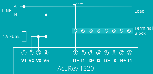
1 ELEMENT 2 WIRE
