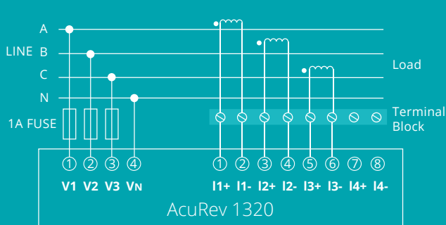
3 ELEMENT 4 WIRE DELTA
