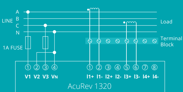
2 ELEMENT 3 WIRE NETWORK
