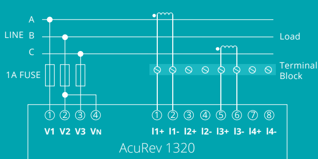
2 ELEMENT 3 WIRE DELTA
