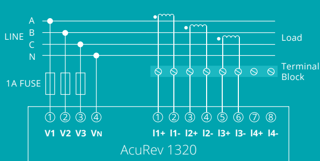
3 ELEMENT 4 WIRE WYE
