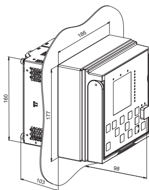
Figure 21. Semi-flush mounting
