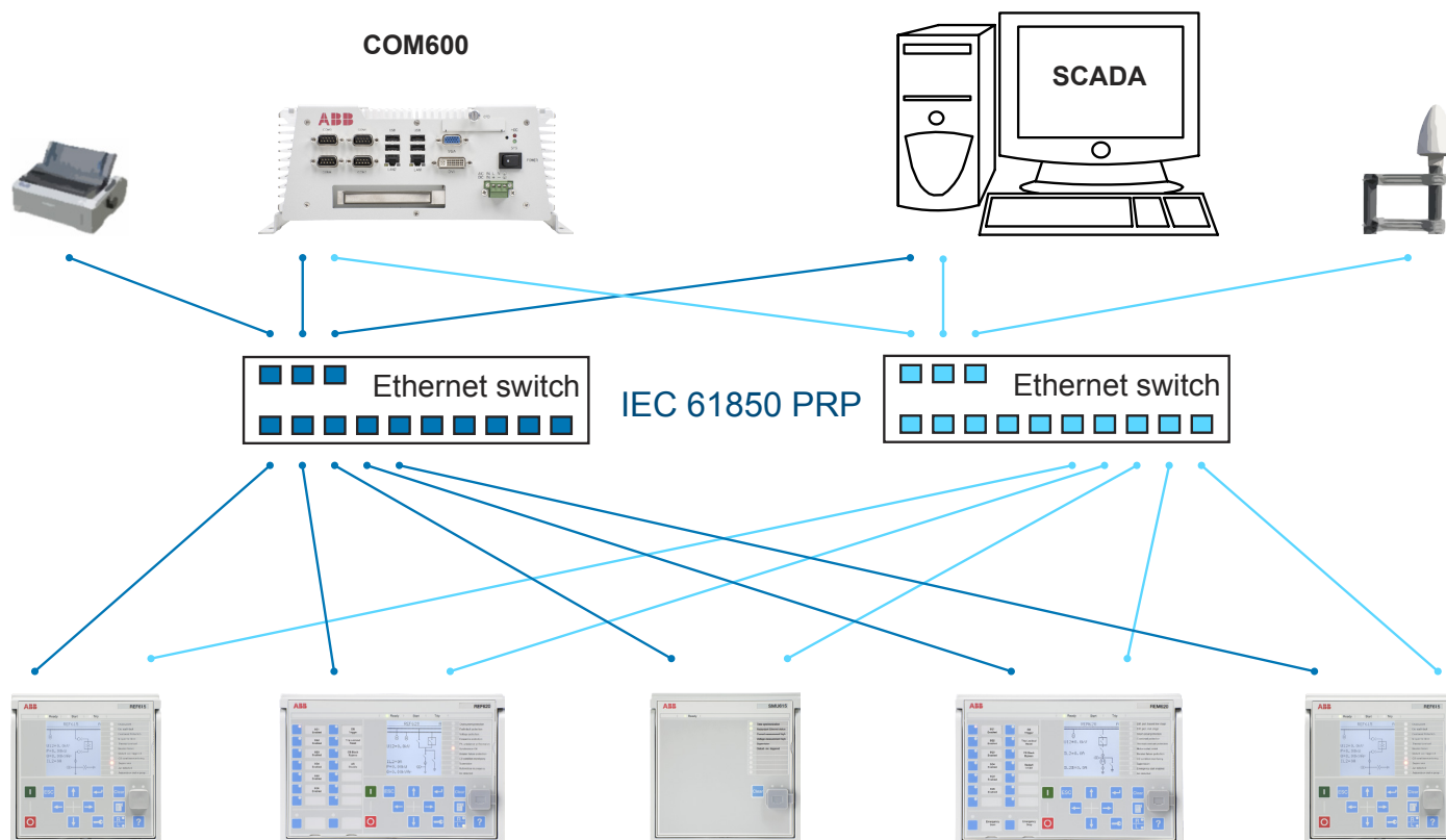
Figure 15. Parallel redundancy protocol (PRP) solution
