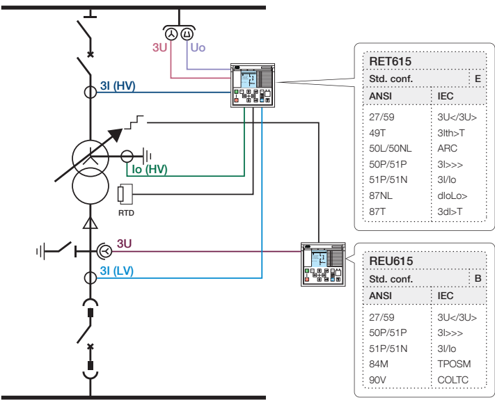
Figure 12. Protection of a two-winding power transformer with RET615 standard configuration E
