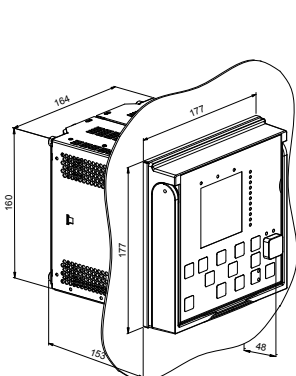
Figure 14: Flush mounting
