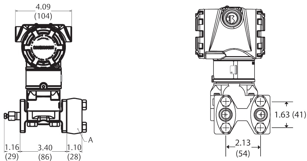
Figure 12: Rosemount 3051C Coplanar with Traditional Flange
