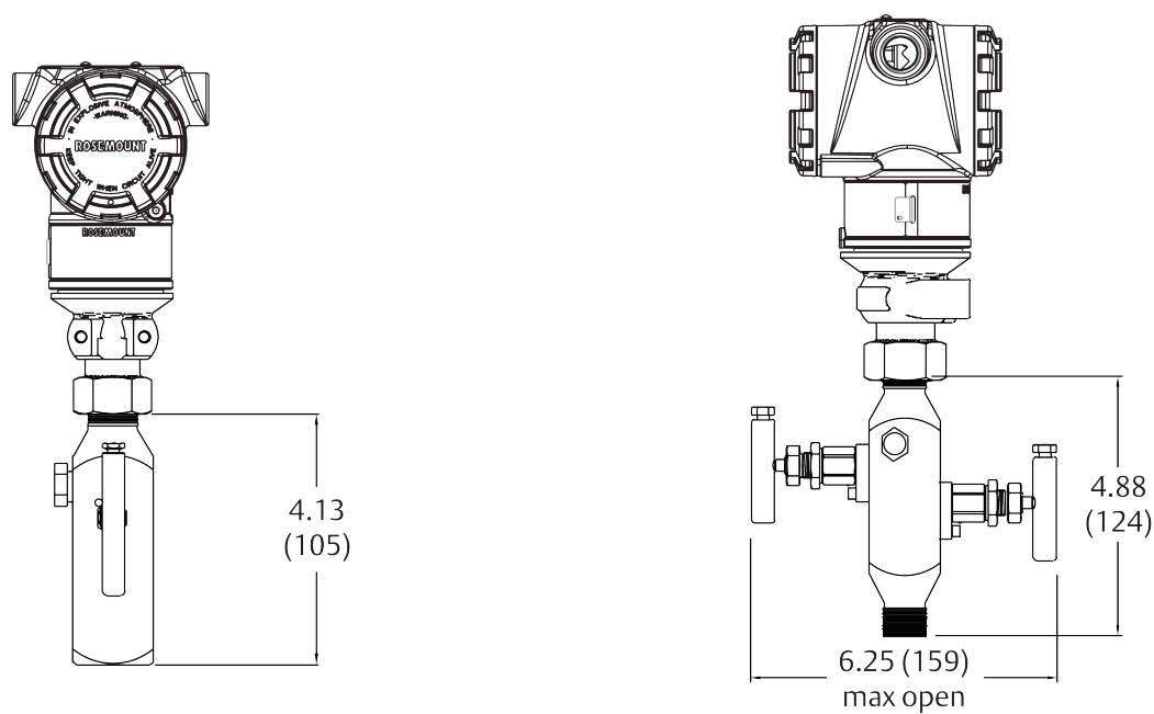
Figure 18: Rosemount 3051T with Rosemount 306 2-Valve Integral Manifold
