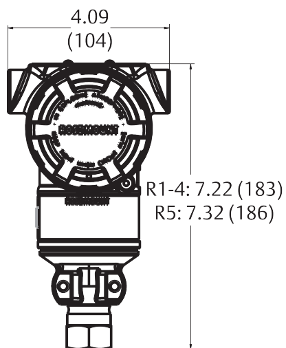
Figure 16: Rosemount 3051T Wireless Housing
