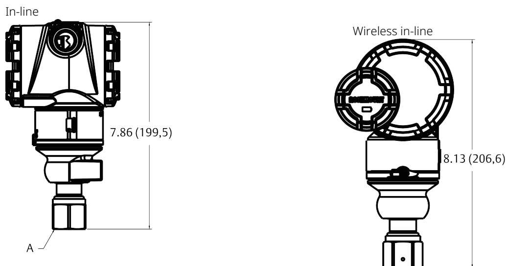
Figure 17: Rosemount 3051T In-Line Range 6
