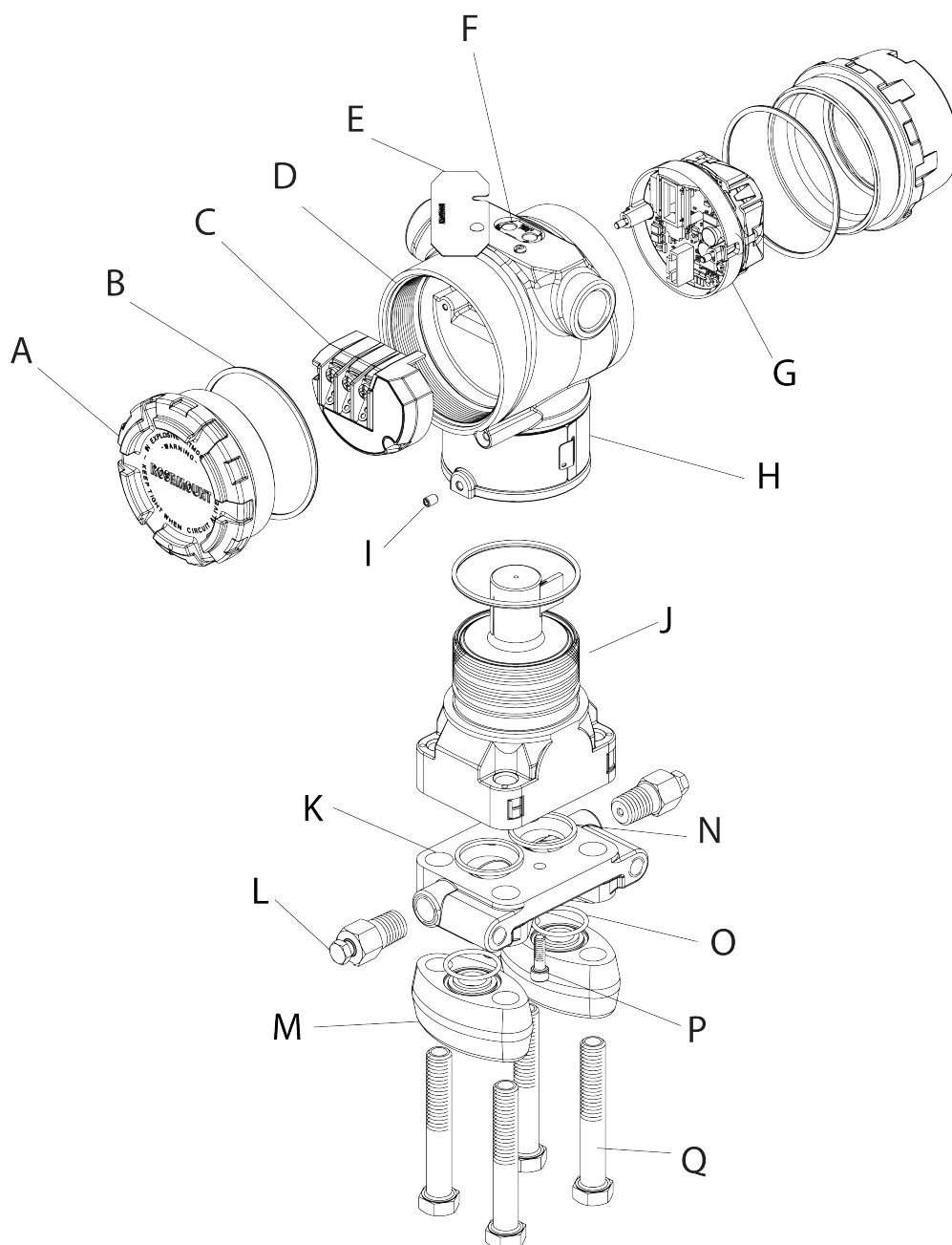
Figure 7: Rosemount 3051C Exploded View
