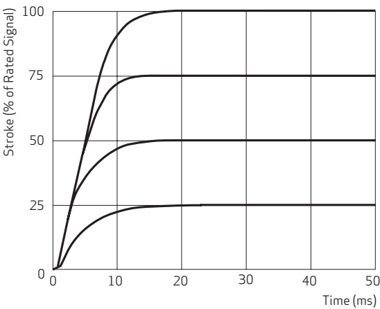
Step Response
