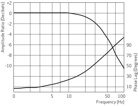
Standard Frequency Response 3,000PSI DTE -24 at 38° C (100° F) ±25% Input Amplitude
