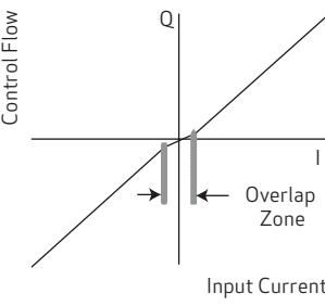
Closed Center Spool Valves
