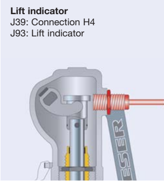
Lift stopper J51
