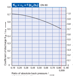
Diagram for evaluation of the coefficient of discharge ( K_{dr}/\alpha_w ) or K_b in reference with the ratio of absolute back pressure / set pressure ( p_{a0}/p_0 )
