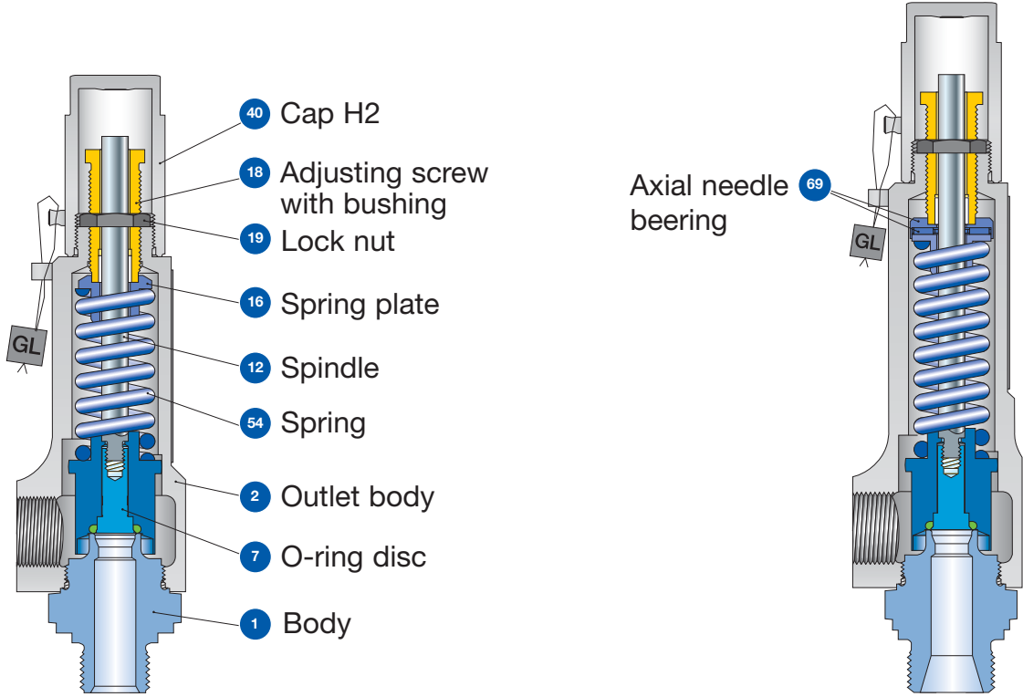
Conventional design Threaded connection
