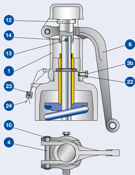
Plain lever H3
