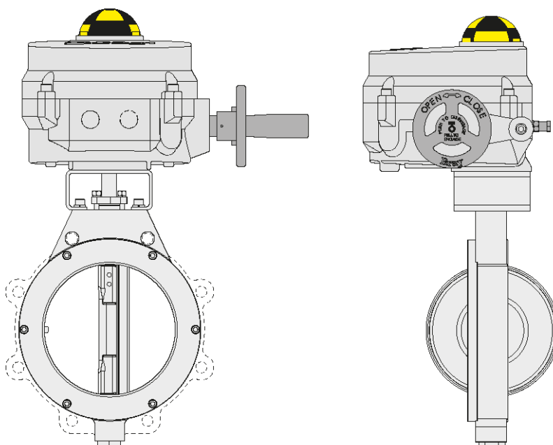
Figure 16: Overall dimensions, in. (mm) for Industrial-Grade VA-9070 Series Electric Actuated Two-Way VF Series High-Pressure, High Temperature Butterfly Valves (see Table 19 and Table 20 )
