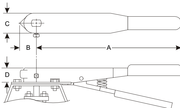
Figure 12: Dimensions for ten-position manual handles
