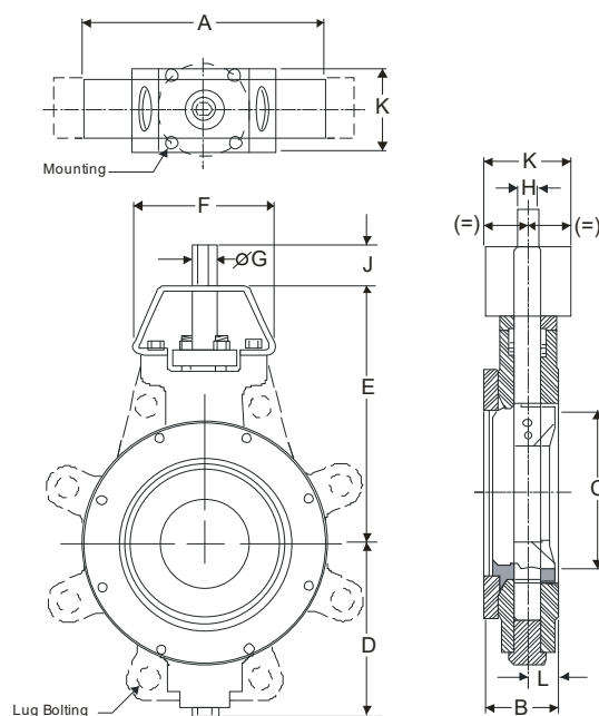
Figure 14: Two-Way VF Series High-Pressure, High-Temperature Butterfly Valve Dimensions (see Table 12 and Table 13 )
