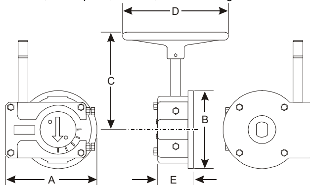
Figure 13: Dimensions for gear-operated manual hand wheels
