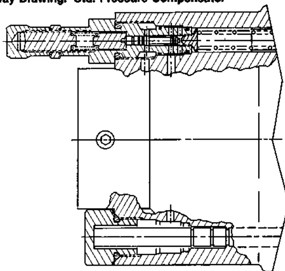
Cutaway Drawing: Std. Pressure Compensator
