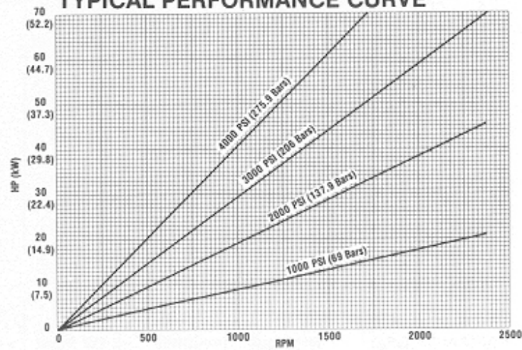
PF 400 FIXED DISPLACEMENT PUMP TYPICAL PERFORMANCE CURVE
