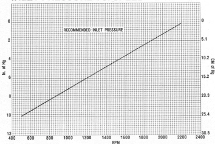
PF 400 SERIES AXIAL PISTON PUMP INLET PRESSURE VS. SPEED
