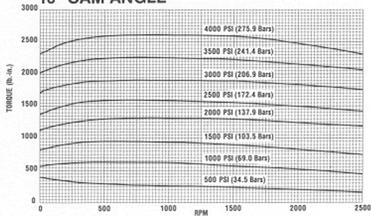
MF 400 FIXED DISPLACEMENT MOTOR 18° CAM ANGLE
