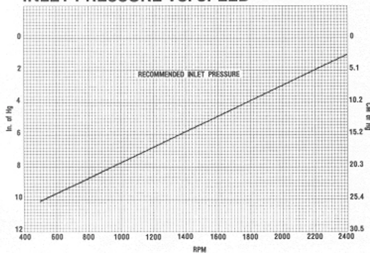
PF 300 SERIES AXIAL PISTON PUMP INLET PRESSURE VS. SPEED
