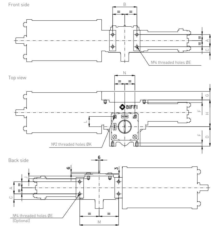
Actuator shown in closed position
