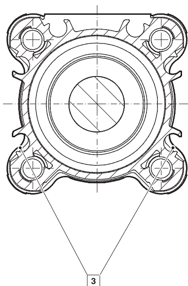
Model Profile barrel ø 32 ... 125 mm
