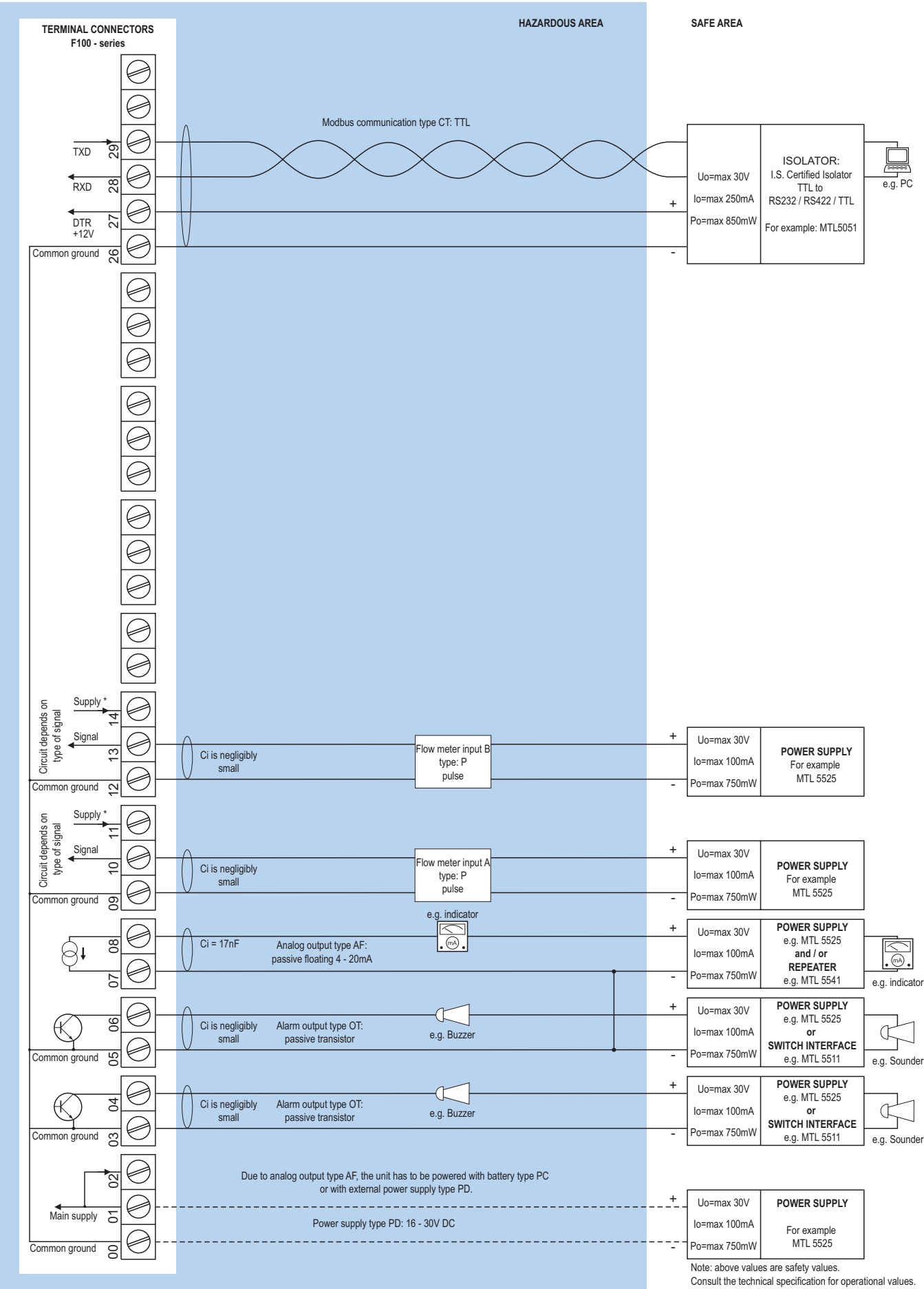
Configuration example IIB / IIIC and IIC - F114-P-AP-(CT)-OT-(PX)-XI - Output loop power
