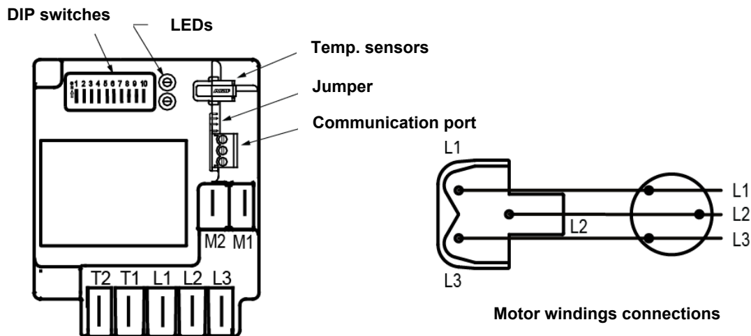
Figure 26: Compressor terminal box wiring with CoreSense Communications module
