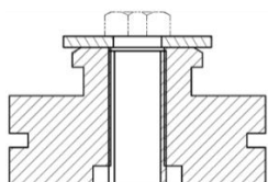
Figure 5: Mounting parts with sleeves and washers
