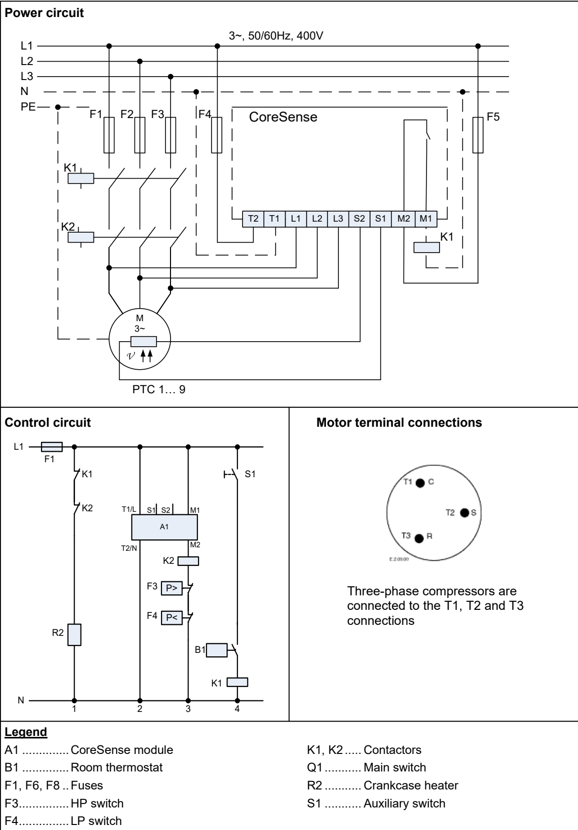
Figure 19: Wiring diagrams for three-phase compressors with CoreSense Communications module
