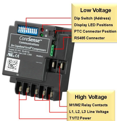
Figure 25: CoreSense Communications module
