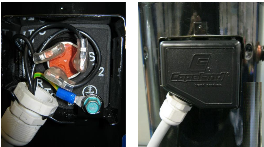
Figure 21: ZP24K* - Electrical installation with cable glands, terminal box IP21
