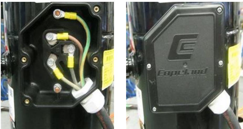
Figure 22: Electrical installation with cable glands, terminal box IP54
