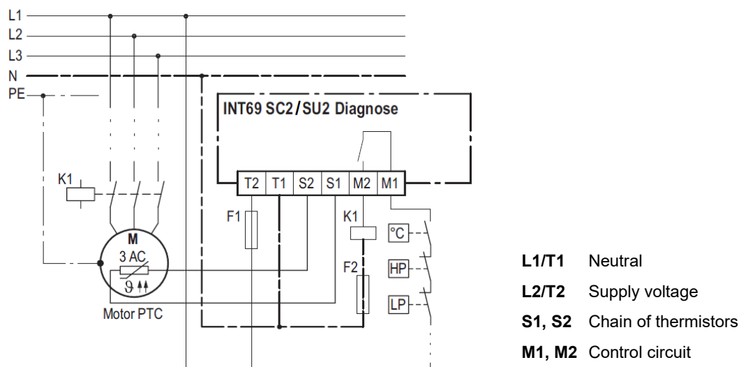
Figure 24: Wiring of the motor protection module
