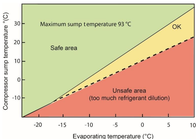
Figure 15: Dilution chart for transient operation
