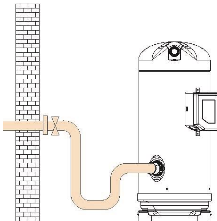
Figure 14: Suction tube design
