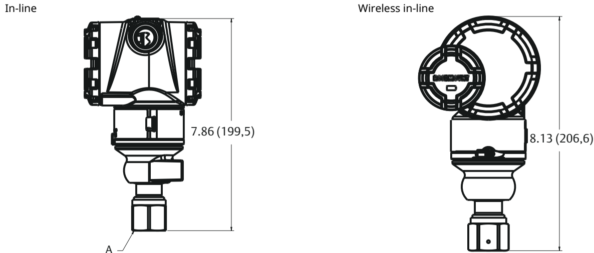
Figure 17: Rosemount 3051T In-Line Range 6
