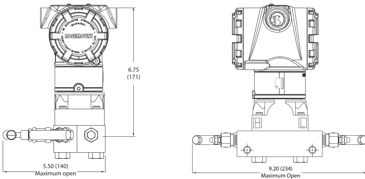
Figure 10: Rosemount 3051C Coplanar Flange with Rosemount 305RC3 3-Valve Coplanar Integral Manifold
