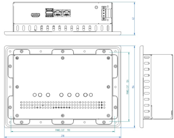
Figure 17 Dimensions External Touch screen 7 inch
