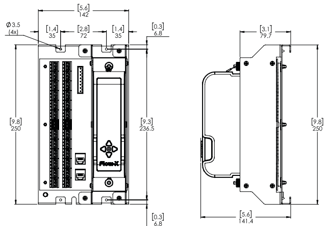
Figure 3 Wall mount
