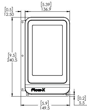
Figure 11 Front view with bracket
