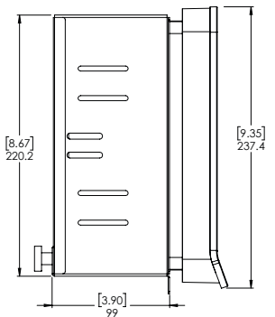
Figure 9 Side view with bracket
