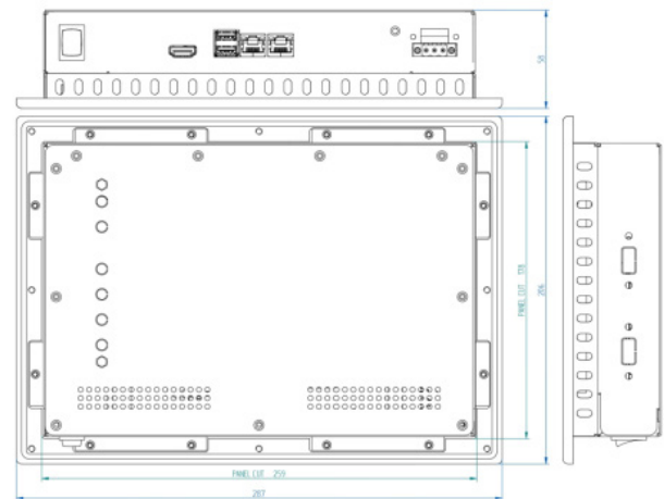
Figure 18 Dimensions External Touch screen 10.1 inch
