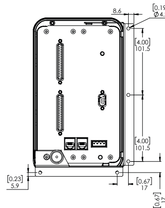
Figure 7 Rear view with bracket
