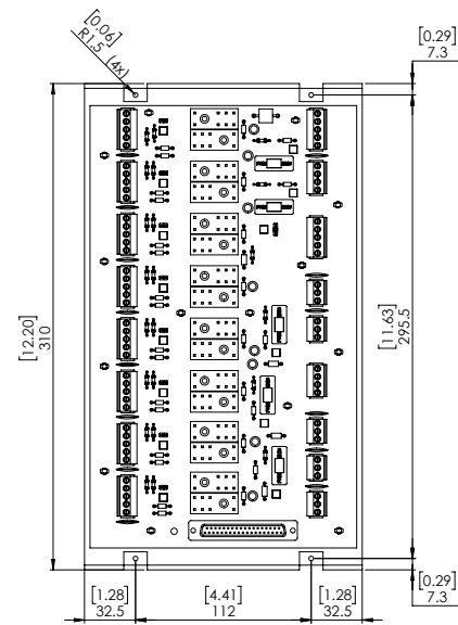
Figure 19 Front view
