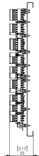
Figure 20 Side view
