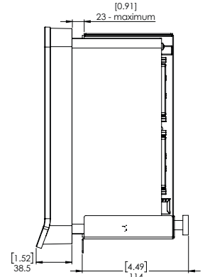
Figure 8 Side view with bracket
