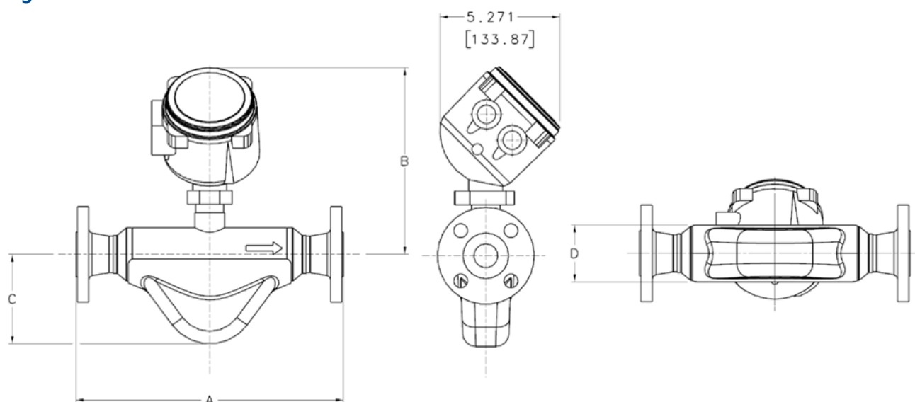
Figure 3: G-Series models dimensions
