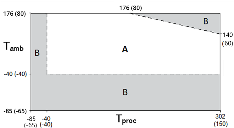
Figure 1: Ambient and process temperature limits for all G-Series meters
