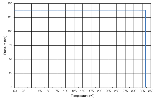
Pressure versus Temperature for C9 Couplers 2
