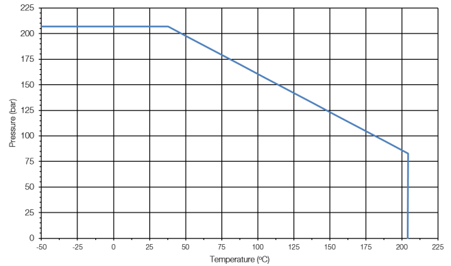
Pressure versus Temperature for C1H and C2H Couplers
