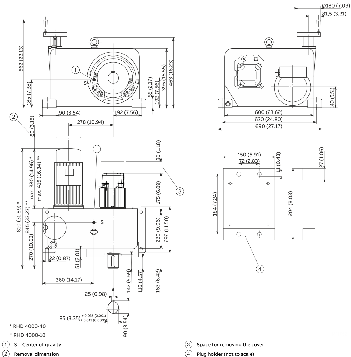
Figure 5: Dimensions in mm (in)
